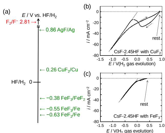
Figure 2. (a) Redox potentials of selected M_xF_x/M ( M : metal) and F_2/F^- couples and cyclic voltammograms of a Ni plate electrode in the CsF-2.45HF molten salt containing (b) CuF_2 and (c) FeF_3 (see Figure S1, Supporting Information, for the cell setup). Metal fluorides were saturated in both the cases. Metal fluorides with redox potentials above HF/H_2 are preferable to avoid H_2 gas generation at the cathode. See Table S1 and related discussion in Supporting Information for thermodynamic estimation of these redox potentials. The potential in the horizontal axis of (b) and (c) is roughly referenced to the potential of H_2 gas evolution by linearly extrapolating the H_2 gas evolution curve. The reduction current of CuF_2 is significantly larger than that of FeF_3 in the range above the H_2 gas evolution potential.
