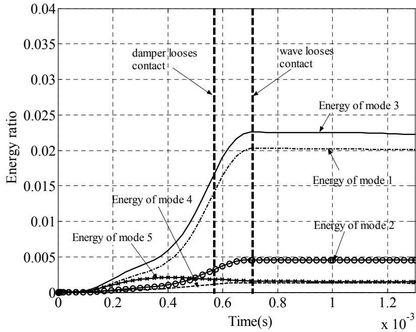
Fig. 5.12 Energy profile of beam mode shape with \omega_w/\omega_1=9 and \omega_d/\omega_1=5 at point P.
