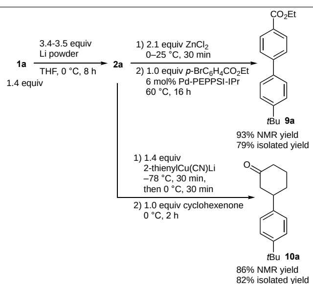
Scheme 3 Reactions of aryllithium 2a via transmetalation.
