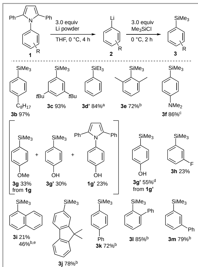
Scheme 2 Reaction scope with respect to the N -aryl group. The efficiency of the lithiation was quantified by determining the yield of the products 3 by ^1\text{H} NMR analysis. a Lithiation and silylation with \text{Et}_3\text{SiCl} were performed at 25 °C. b 0 °C for 1 h and 25 °C for 1 h for the silylation. c Lithiation for 8 h. d Lithiation with 4.0 equiv Li powder at 25 °C and silylation with 4.0 equiv \text{Me}_3\text{SiCl} . e 3.0 equiv Na dispersion and LiI.
