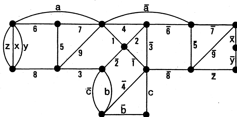
(a) matroid m
