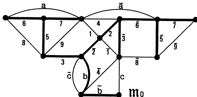
(b) central minor and its parity base
