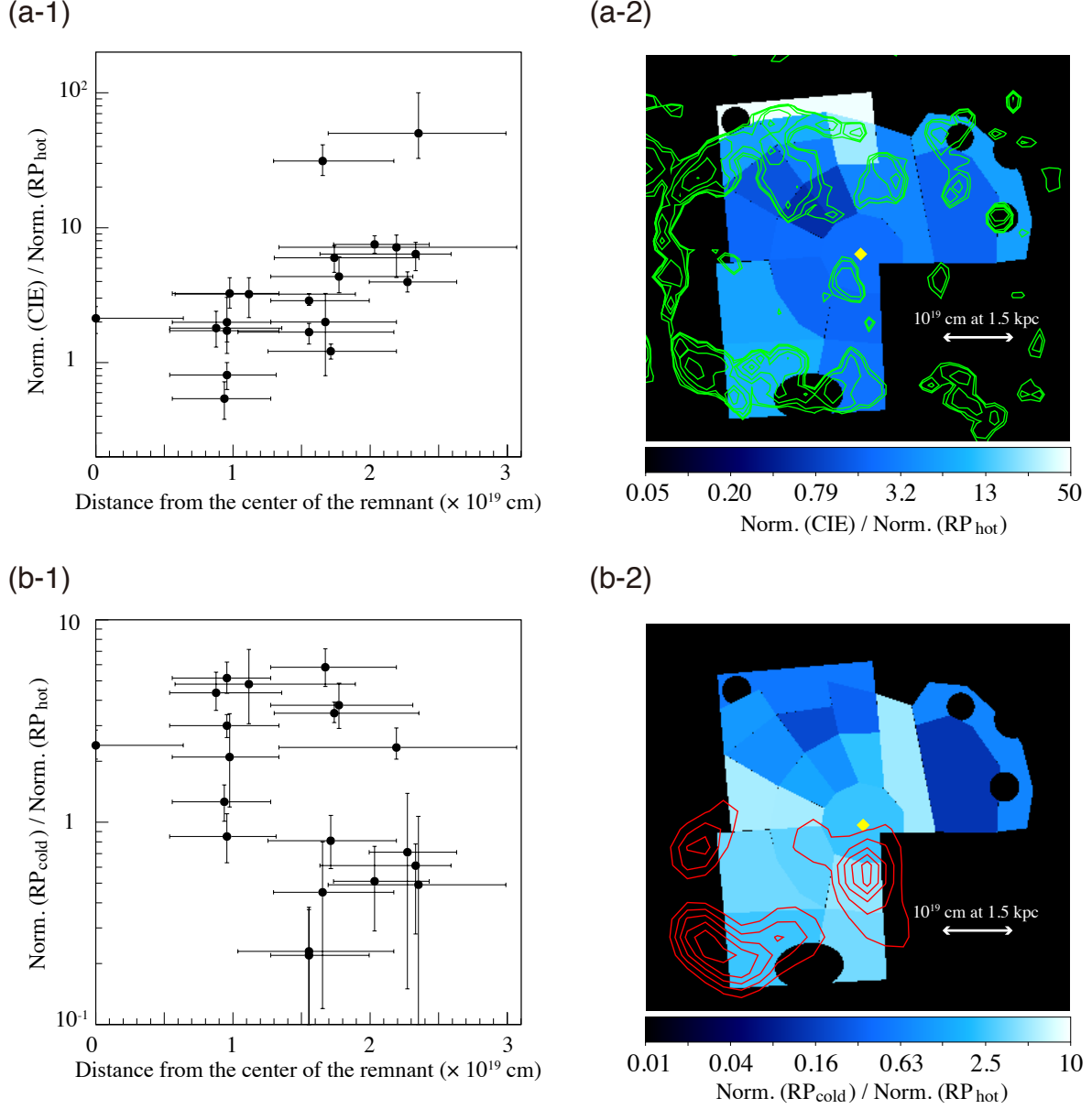
Figure 6.6: (a-1) Radial profile and (a-2) map of the CIE to \text{RP}_{\text{hot}} normalization ratio with the 1.4 GHz radio emissions (green contours). (b-1) Radial profile and (b-2) map of the \text{RP}_{\text{cold}} to \text{RP}_{\text{hot}} normalization ratio with a map of the ^{12}\text{CO}(J=2-1) to ^{12}\text{CO}(J=1-0) intensity ratio (red contours; Yoshiike, 2017). The yellow diamonds denote the center of the remnant (R.A., Dec.) = ( 6^{\text{h}}17^{\text{m}}40^{\text{s}}.0 , 22^{\circ}38'00''.0 ). The length of the white arrows correspond to 10^{19} cm at the distance of 1.5 kpc.
