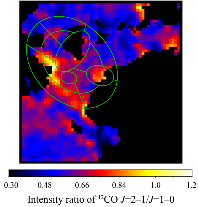
Figure 7.9: Spatial distribution of the intensity ratio of the ^{12}\text{CO}(J = 2-1) to ^{12}\text{CO}(J = 1-0) emissions in the velocity range of 30-40 \text{ km s}^{-1} with the NANTEN2 observations (Yoshiike, 2017). The solid green lines show the regions used for the spectral analysis.
