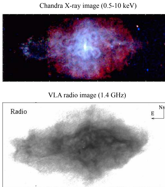
Figure 2.8: X-ray and radio images of the plerionic SNR, 3C 58 (Slane et al., 2004). (upper) X-ray image in the energy band of 0.5-10.0 keV with Chandra. (bottom) 1.4 GHz radio continuum image from with VLA.
