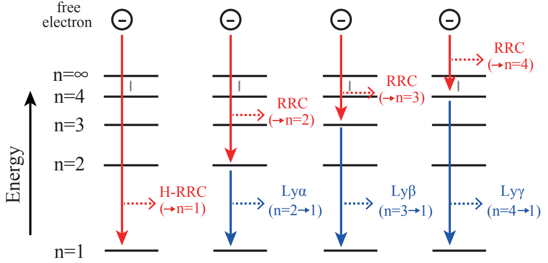
Figure 3.4: Schematic illustration of emission mechanism for radiation recombination continua (red arrows) and cascade lines (blue arrows).
