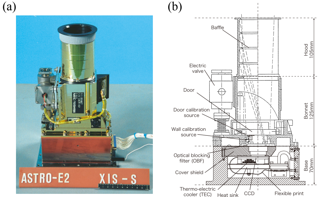
Figure 4.6: (a) Photograph and (b) side view of the XIS (Koyama et al., 2007).
