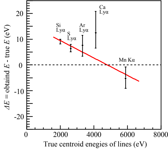
Figure 4.14: Comparison of centroid energies of emission lines from W49B before applying the calibration described in §4.3.3. The red line indicates a function estimated by linear regression.
