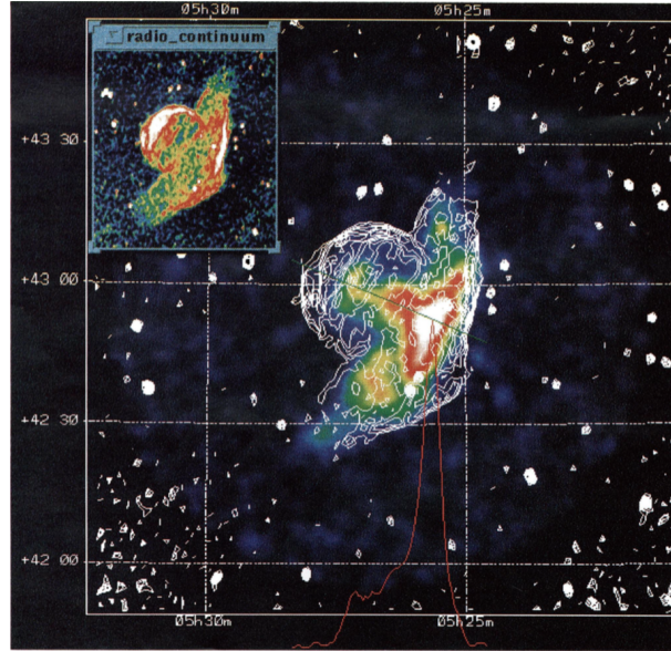
Figure 5.1: ROSAT image of G166.0+4.3 in the 0.52-2.02 keV band with 1.4 GHz radio contours (Burrows & Guo, 1994). The coordinates refer to the J2000.0 epoch. The red curve along the bottom of the image represents the X-ray intensity along the slice shown as a green line, which passes through the center of the SNR near its plane of symmetry. The inset in the upper left-hand corner is a color image of the radio continuum data, scaled from 0 to 1.67 K.
