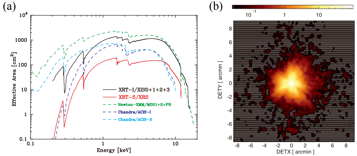
Figure 4.4: (a) Total effective area of the four XRT-I modules with those of XMM-Newton and Chandra. Transmissions of the thermal shield and the optical blocking filter, and the quantum efficiency of the CCD are all taken into account. (b) XIS0 image of a bright point source, SS Cygni. The figures are taken from Serlemitsos et al. (2007)
