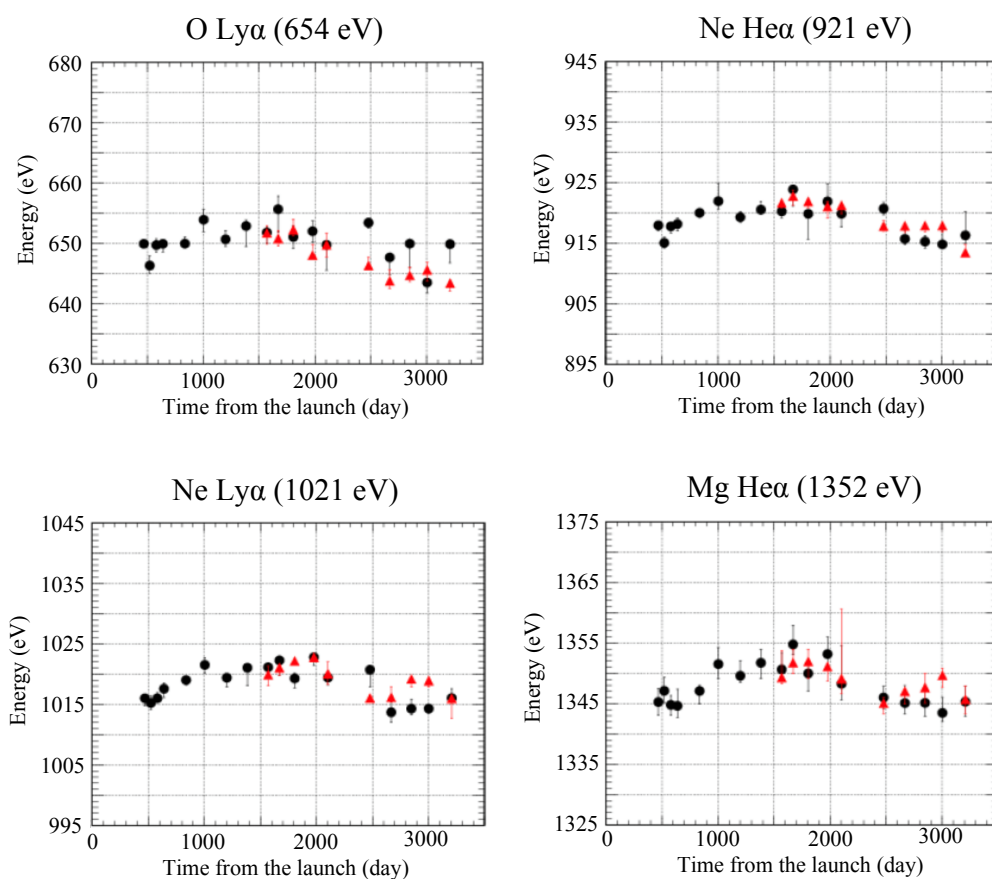
Figure 4.13: Trends of centroid energies of O Ly \alpha , Ne He \alpha , Ne Ly \alpha and Mg He \alpha of E0102–72.3 obtained with XIS0. The black and red points are data taken in readout modes with no option and with the 1/4 window option (for a bright source), respectively (Suzaku Technical Description).
