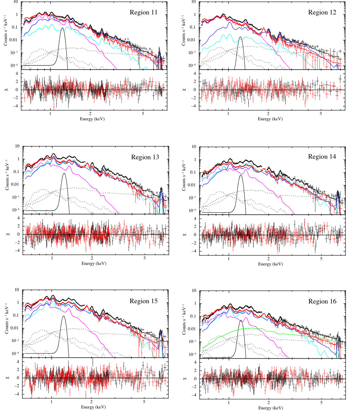
Figure A.4: Same as Figure 6.4 but for regions 11–16.
