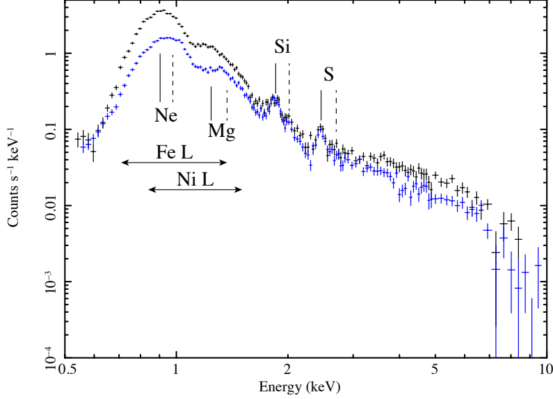
Figure 5.4: XIS0+3 spectra of the W (black) and NE (blue) regions. The vertical solid and dashed black lines show the center energies of the K lines from He-like and H-like ions, respectively. The arrows indicate the energy bands with Fe-L and Ni-L line complexes.
