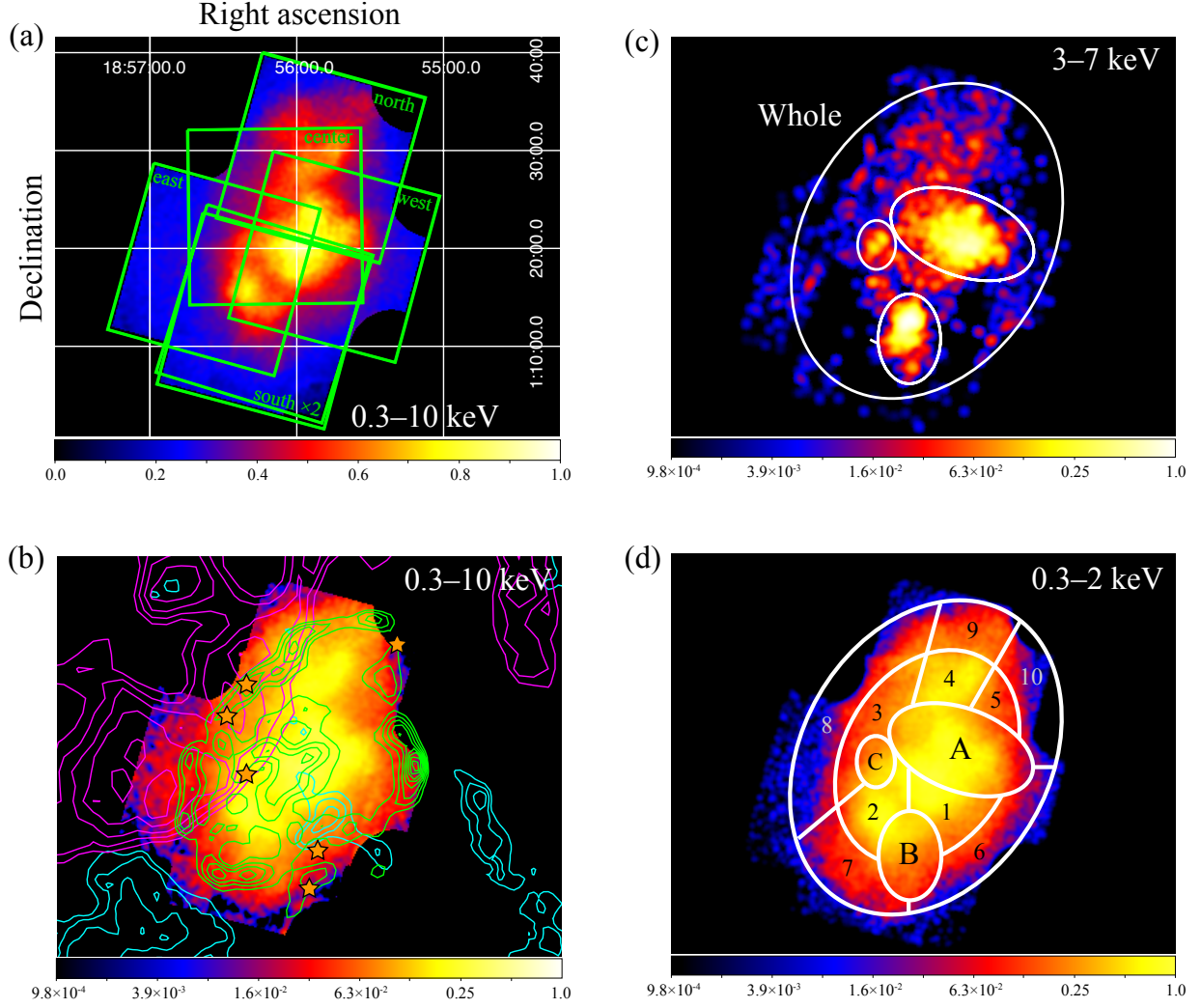
Figure 7.1: XIS3 images of W44 in the energy band of (a,b) 0.3–10 keV, (c) 3–7 keV and (d) 0.3–2 keV after the NXB subtraction and correction for the vignetting effect. The X-ray count rates are normalized so that the peaks become unity. In panel (a), the green squares are the FOVs of XIS3 in each observation. The coordinate refers to the J2000.0 epoch. In panel (b), the green contours are a radio image as seen in 20 cm wavelength by the Very Large Array (VLA) (Helfand et al., 2006). The magenta and cyan contours are the NANTEN2 ^{12}\text{CO}(J = 2-1) images in the velocity range of 40–50 km s ^{-1} and 50–60 km s ^{-1} , respectively (Uchida et al., 2012). The orange stars indicate the locations of the 1720 MHz OH maser emissions (Claussen et al., 1997). The white lines in panels (c) and (d) indicate regions for the spectral extraction.
