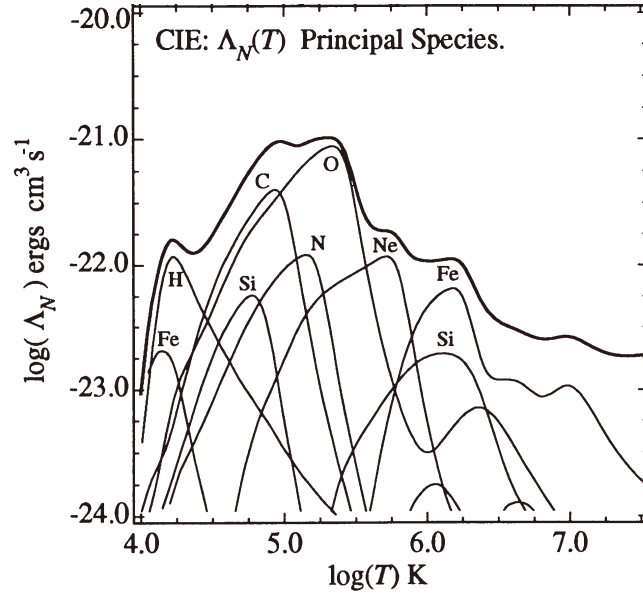
Figure 2.6: Cooling coefficient for an optically-thin thermal plasma with solar abundances (Anders & Grevesse, 1989) as a function of plasma temperature (Sutherland & Dopita, 1993).
