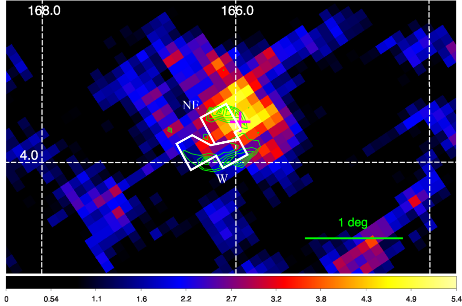
Figure 5.9: Signal-to-noise map in the G166.0+4.3 smoothed with a boxcar of length 0^\circ.5 in the energy band of 0.5–2 GeV with Fermi (Araya, 2013). The green contours show the WENSS 325 MHz radio image. The white lines indicate the NE and W regions. The Galactic coordinates are referred.
