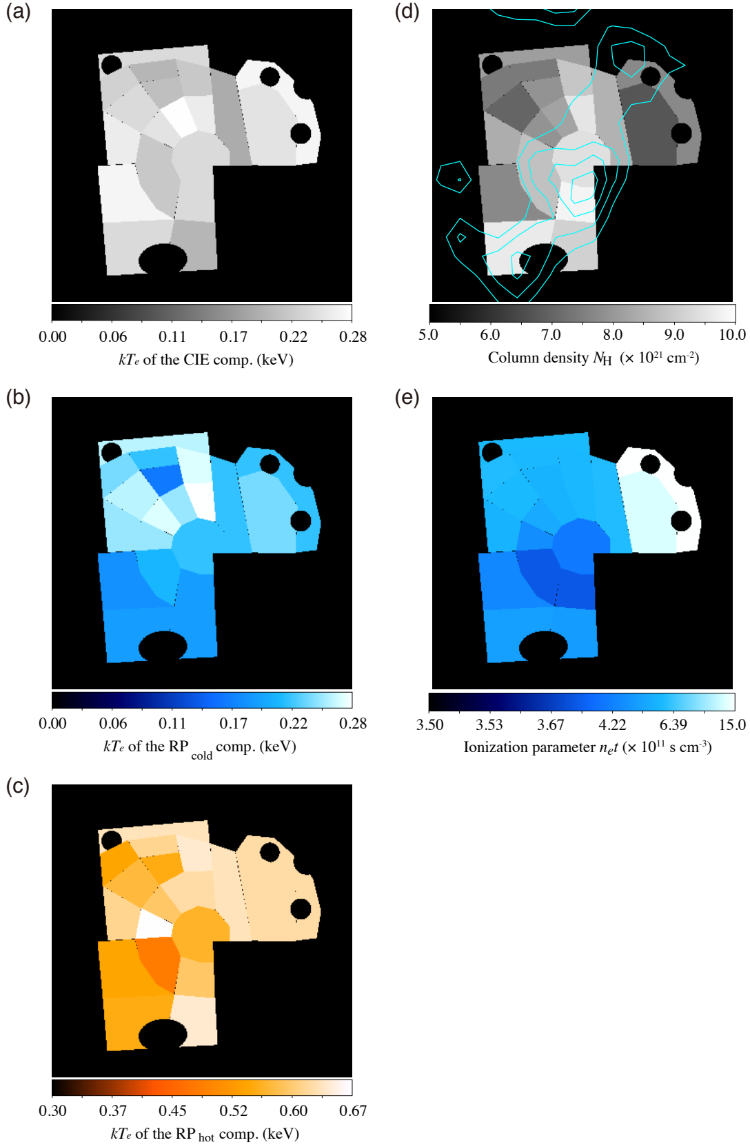
Figure 6.5: (a–c) Maps of the electron temperatures kT_e of the CIE, \text{RP}_{\text{cold}} , \text{RP}_{\text{hot}} components. (d) Map of the column density N_{\text{H}} with the ^{12}\text{CO}(J = 1 - 0) emissions (cyan contours; Yoshiike, 2017). (e) Map of the ionization parameters n_e t .
