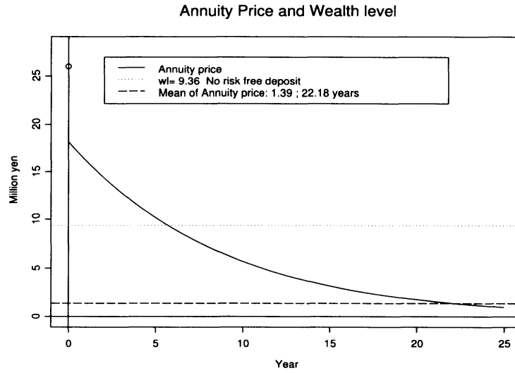
Figure 4: Mean time of purchasing annuity
