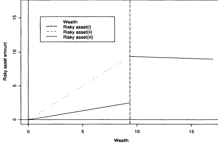
Figure 2: Optimal Investment: Risky & Riskless assets
