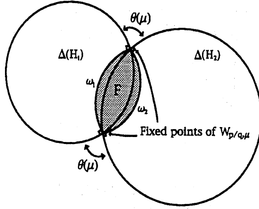
Figure 3: The set F .
