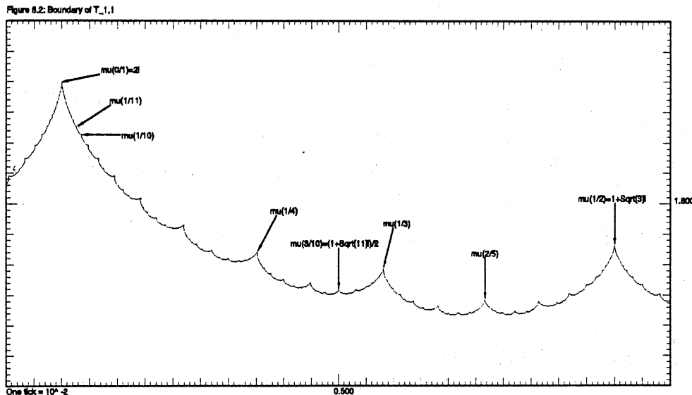
Figure 1: The Maskit embedding Courtesy of David J. Wright
