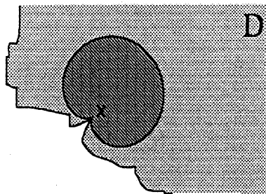
Figure 2: An inward-pointing cusp.
