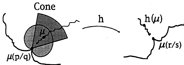
Figure 4: A cone with vertex at \mu(p/q)
