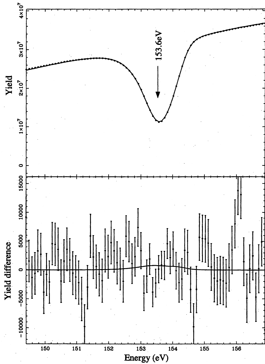
Figure B.12: The spectrum around the 153.6-eV resonance. The resonance shows no parity violating asymmetry within statistical error.
