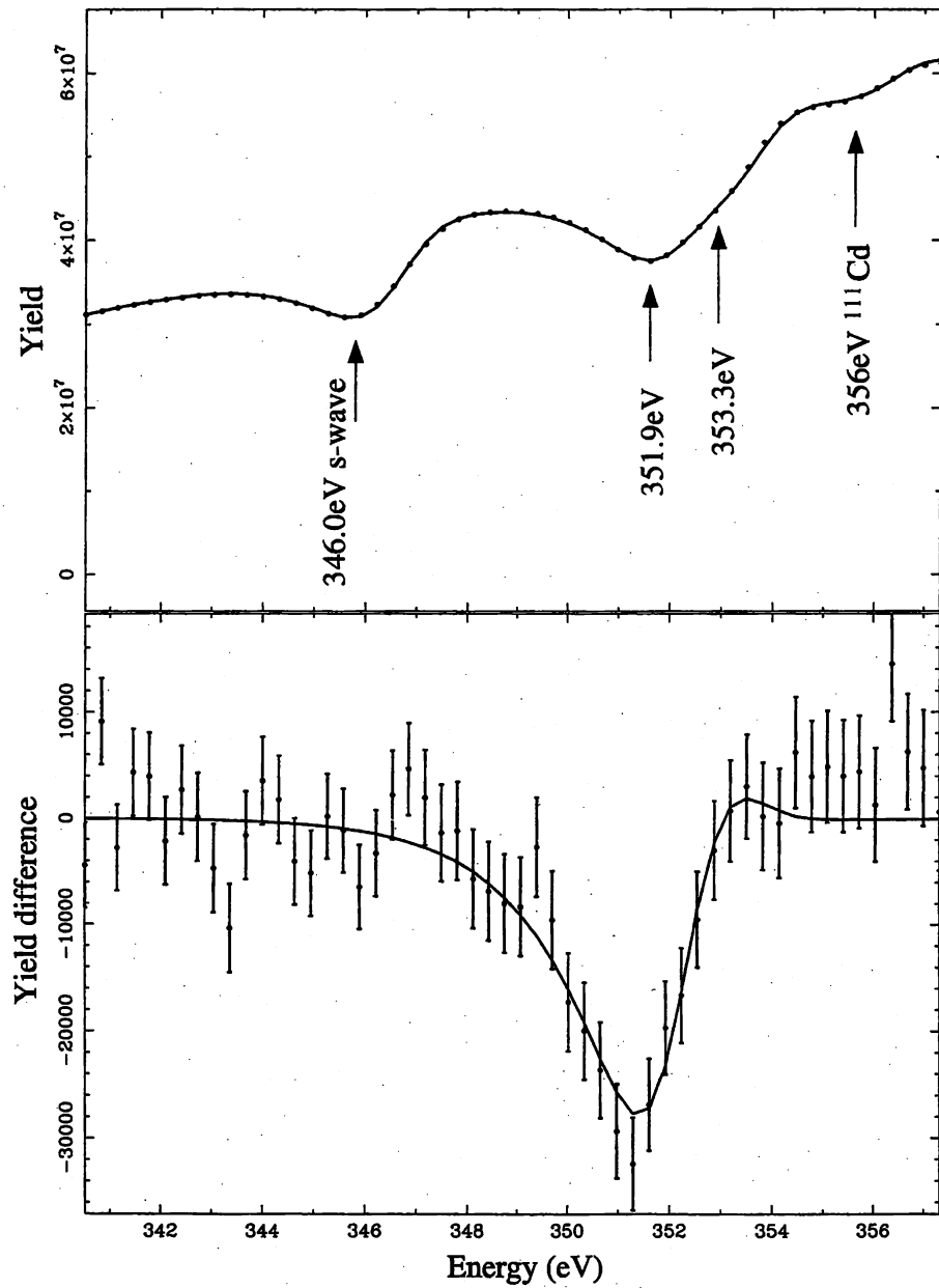
Figure B.16: The spectrum around the 351.9-eV and 353.3-eV resonances. Two resonances are overlapping in the neutron transmission spectrum (shown in upper graph), but the difference of the transmission spectra shows that the 351.9-eV resonance has a large asymmetry whose significance is 8.4\sigma whereas the 353.3-eV resonance has no asymmetry within statistical error.
