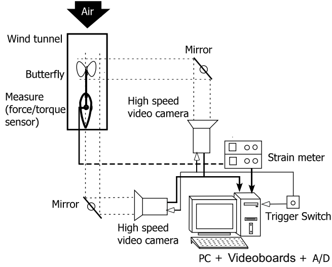
Figure 4: Experimental setup
