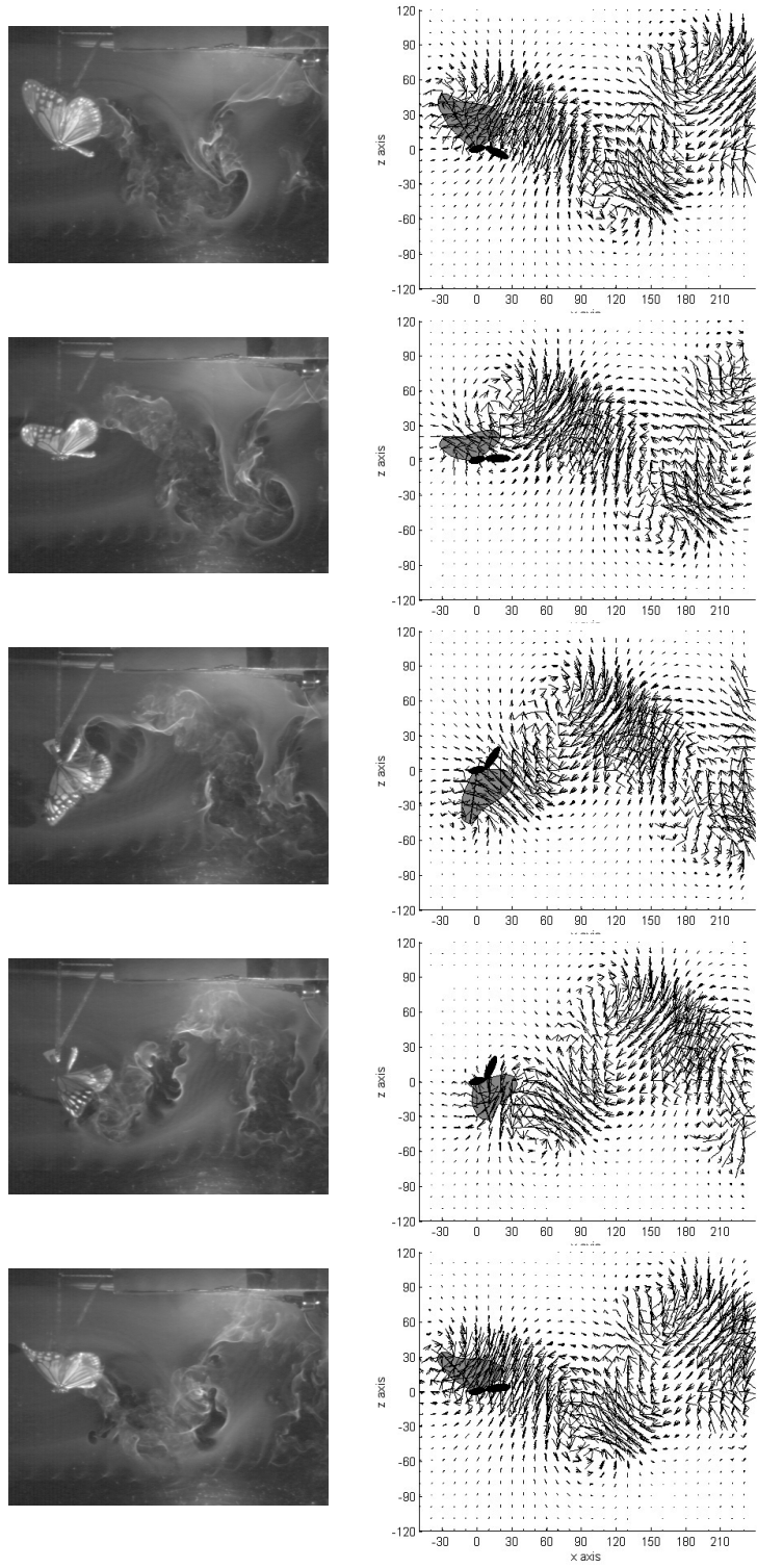
Figure 7: Comparison of flow fields of experimental visualization and numerical simulation by panel method every 0.036 s. ( V = 1.0 m/s, \theta_t = -10^\circ )
