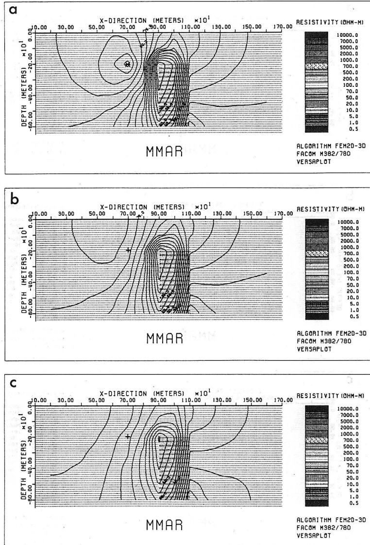
Fig. 5. Apparent resistivity contour sections normalized by the nontarget inhomogeneities model (Model 71W, \rho_1=\rho_3=700 ohm-m, \rho_2=100 ohm-m and \rho_4=200 ohm-m in Fig. 3). (a) : xz section with the source C(I), (b) : xz section at the distance 200m from C(I), (c) : xz section at the distance 400m from C(I).
