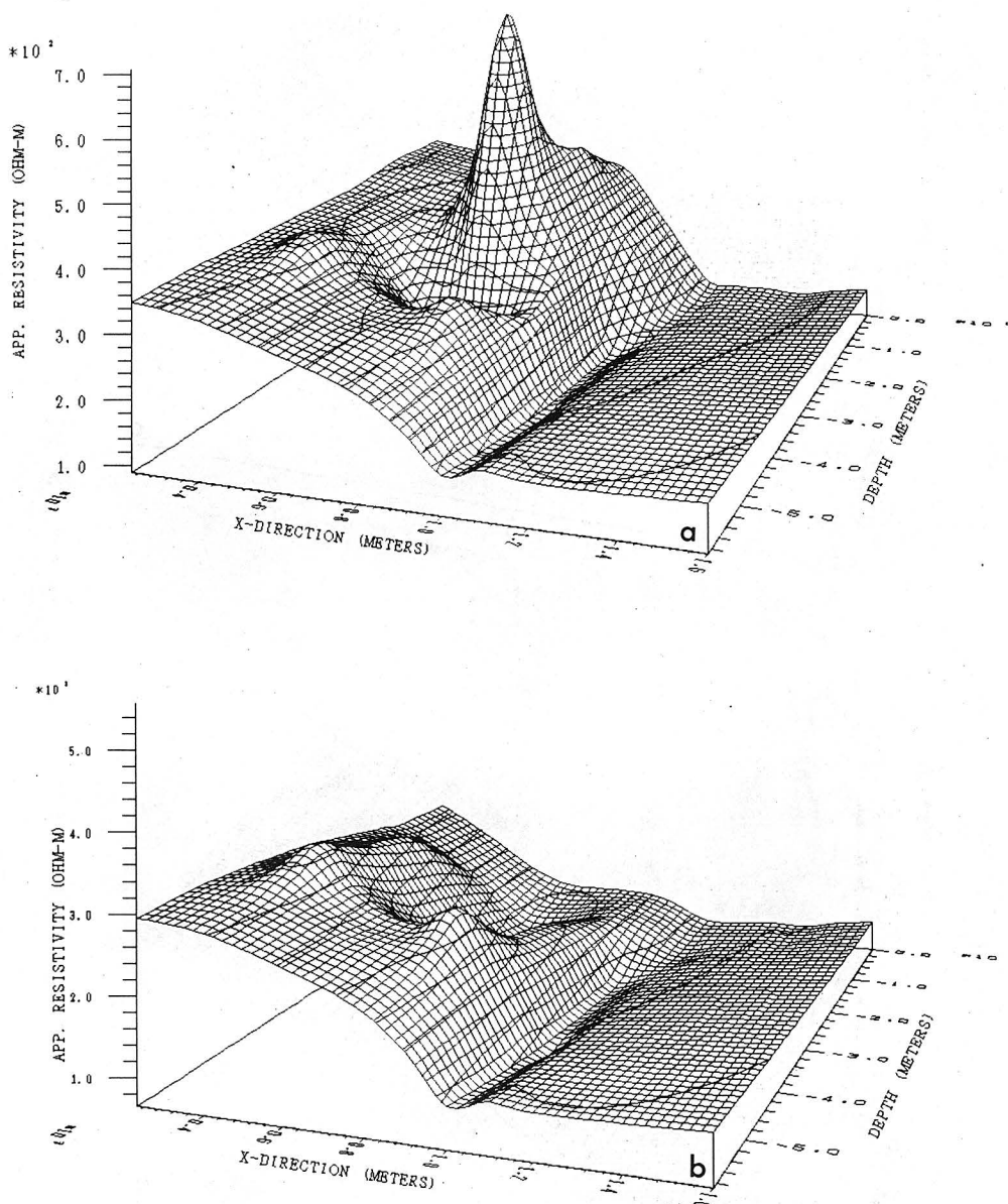
Fig.9. Apparent resistivity three-dimensional perspective views of plot. (a): Perspective view of Figure 8a (Model 5272WLN), (b): Perspective view of Figure 8b(Model 5272WLC).
