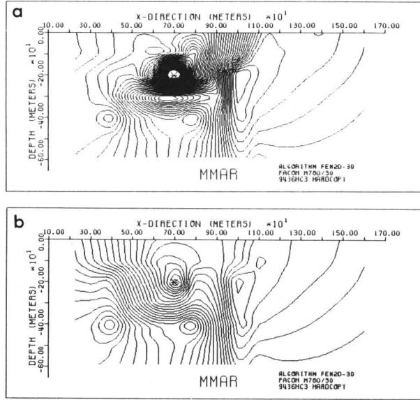
Fig.8. C(subsurface) P(subsurface) cross-hole apparent resistivity contour sections. (a): Model 5272WLN ( \rho_1=\rho_9=700 ohm-m, \rho_2=\rho_4=200 ohm-m, \rho_3=10 ohm-m, \rho_5=1000 ohm-m, \rho_6=100 ohm-m, \rho_7=500 ohm-m, \rho_8=20 ohm-m and \rho_9=700 ohm-m in Fig.7), (b): Model 5272WLC (same as Model 5272WLN except \rho_9=20 ohm-m in Fig.7).
