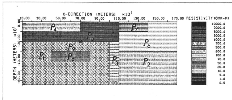
Fig.7. An example of complicated resistivity model which consists of a conductive vertical target and its surroundings including a vertical contact, partial horizontal overburden, a deep horizontal layer, near-surface local inhomogeneity and local structure near the source C(I).
