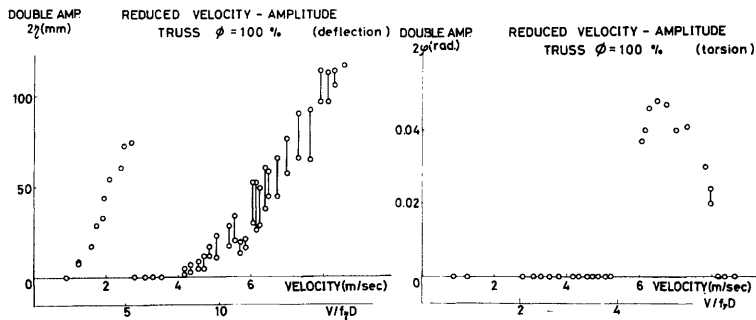
Fig. 16. Measured amplitude. (Truss Section)
