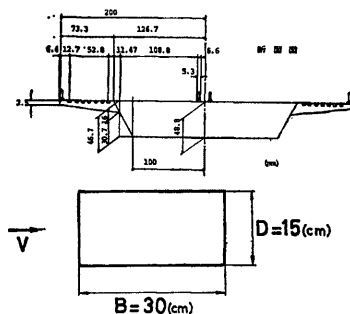
Fig. 1. Cross section (Box-Girder and Rectangular 1:2).
