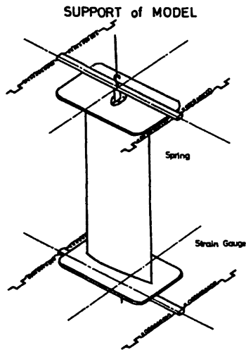
Fig. 2. Sketch of supported model.
