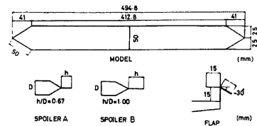
Fig. 13. Hexagonal Box-Girder, Spoiler and Flap plate
