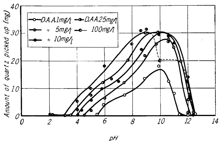
Fig. 21. Flotation curves for quartz in solutions of various concentrations of dodecyl ammonium acetate.
