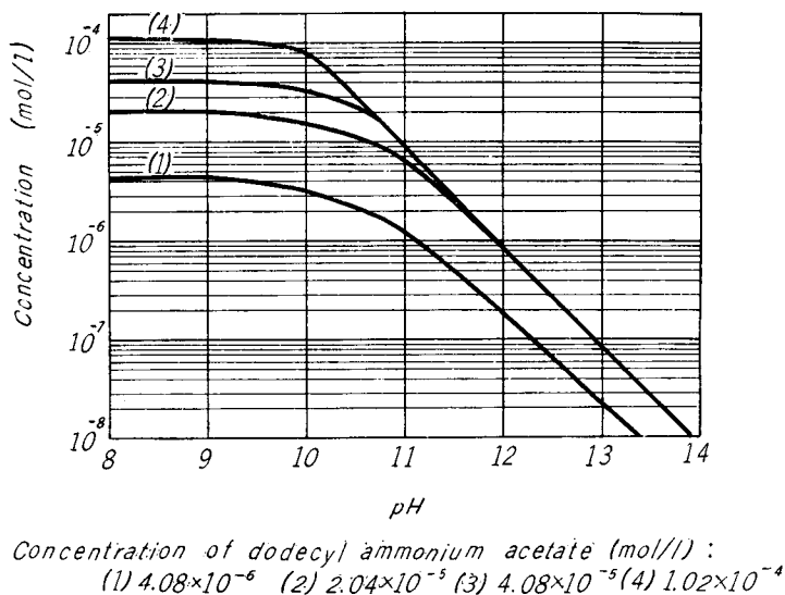
Fig. 7. Relation between pH value and dodecyl ammonium ion concentration.
