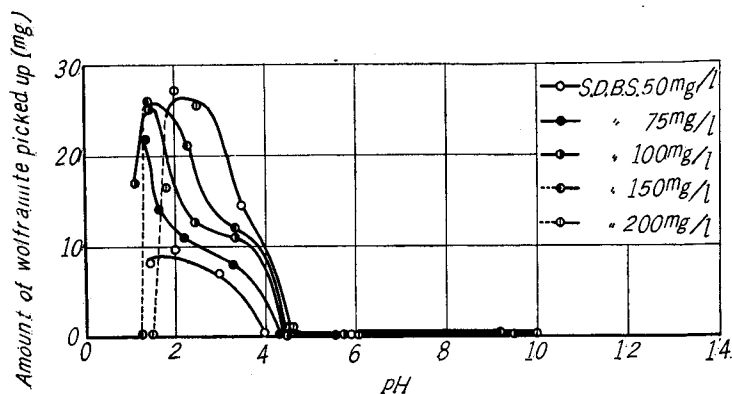
Fig. 10. Flotation curves for wolframite in solutions of various concentrations of sodium dodecyl benzene sulphonate.
