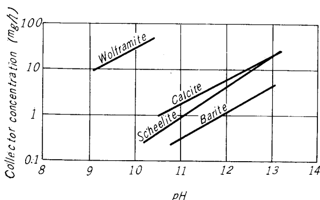
Fig. 20. Relation between concentration of sodium oleate and critical pH value.
