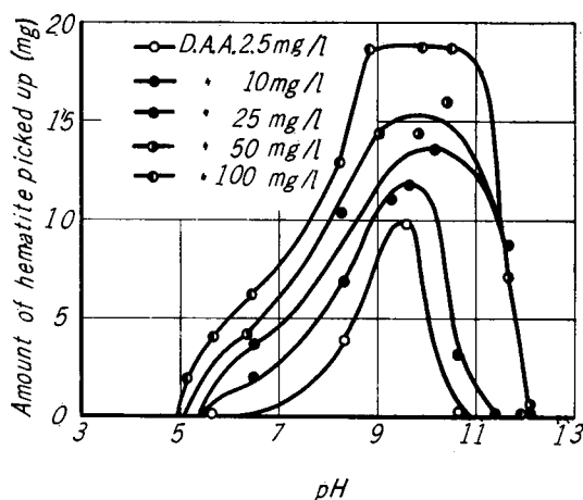
Fig. 2. Flotation curves for hematite in solutions of various concentrations of dodecyl ammonium acetate.
