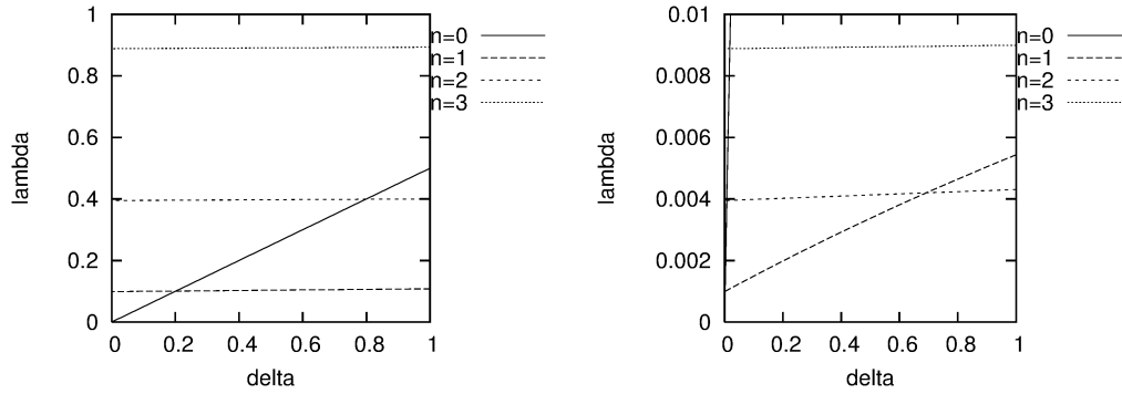
Figure 1. Hopf bifurcation curves in (\delta, \lambda) -plane. Parameter: \varepsilon = 0.01 (left), \varepsilon = 0.0001 (right).
