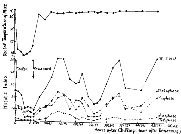
Fig. 21 Changes in mitotic index in Ehrlich solid carcinoma from mice subjected to 6 hours hypothermia at 20^{\circ}\pm 2^{\circ}\text{C} .
