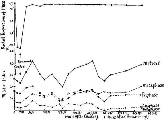
Fig. 15 Changes in mitotic index in Sarcoma 180 solid tumor from mice subjected to 2 hours hypothermia at 20^{\circ} \pm 2^{\circ}\text{C} .
