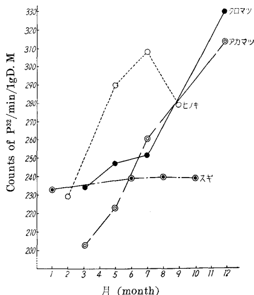
Fig. 1 Seasonal Variation of Counts of P^{32} /min/1g D. M. of Sugi Seedlings cultivated in normal culture Solution.
