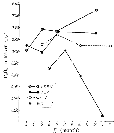
Fig. 2 磷酸含有率季節的变化 Seasonal Variation of P_2O_5 in Needles of several species
