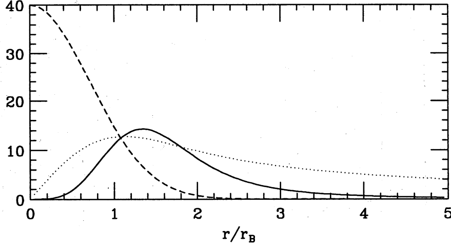
Figure 1: Dashed line, the axial vorticity \omega ; dotted line, the azimuthal velocity v_\theta ; solid line, the local energy dissipation rate \varepsilon_{\text{loc}} of the Burgers' vortex. r_B = 1 , \nu = 0.1 and R_\Gamma \equiv \Gamma/\nu = 1257 .
