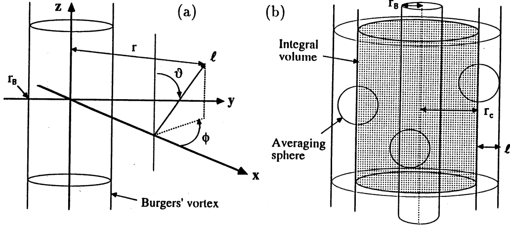
Figure 2: (a) The coordinate system at spherical average with respect to the running point \mathbf{x} + \boldsymbol{\ell} where the reference point \mathbf{x} and the separation length \ell are fixed. (b) The integral space with respect to the reference point \mathbf{x} .
