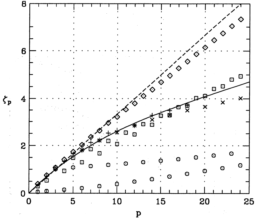
Figure 4: The exponent \zeta_p of the structure function S_p shown by \diamond , \square and \odot which are as in figure 3. dashed line, K41 (1.13); solid line, log-Poisson model (1.17); \times , DNS at R_\lambda = 150 , Vincent & Meneguzzi (1991) [1]; + , jet at R_\lambda = 852 , Anselmet et al. (1984) [11].
