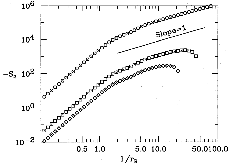
Figure 3: The 3rd-order structure function times -1. \diamond , R_\Gamma = 628 ; \square , R_\Gamma = 1257 ; and \odot , R_\Gamma = 12566 .
