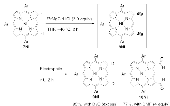
Scheme 1. Dimagnesiation of \beta,\beta' -diiodoporphyrin 7Ni
