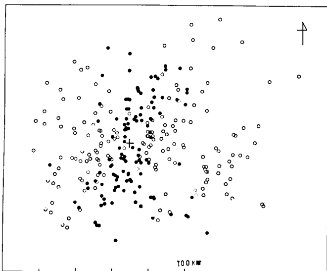
Fig. 5. The first motions of P waves of microearthquakes, \bullet , condensation, \circ ; rarefaction, + ; epicenter.
