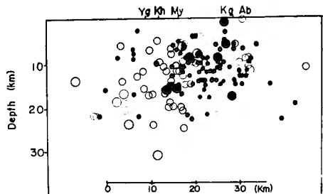
Fig. 4. Distribution of the depths of earthquakes with their magnitude class.
