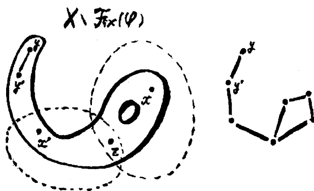
Figure 13: Realization of Čech Complex
