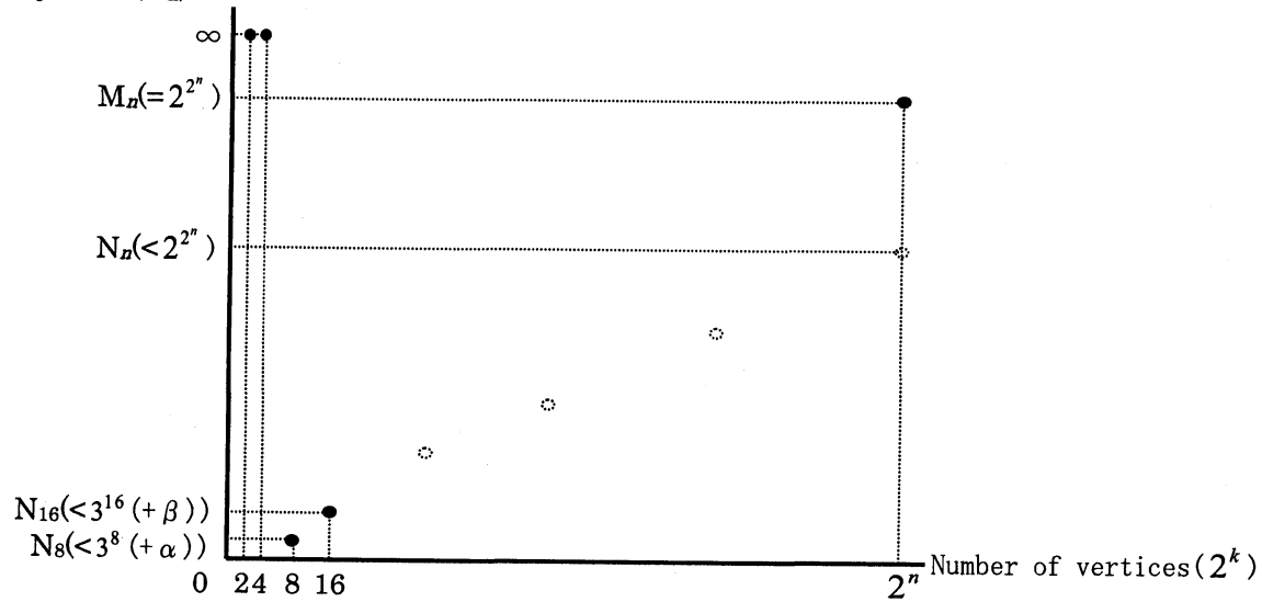
Distribution of the Sequences (assumption, by single logarithmic chart)
