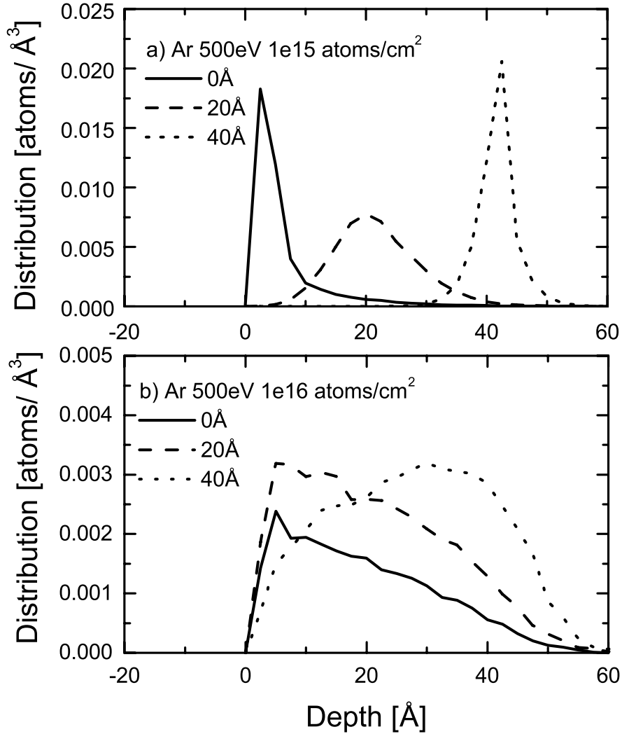
Fig. 4: Distribution of marker atoms calculated by T-DYN. The incident energy is 500eV and the atomic dose is (a) 1.0 \times 10^{15} /cm 2 and (b) 1.0 \times 10^{16} /cm 2 .
