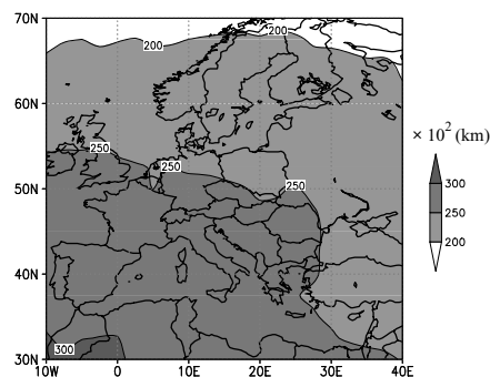
Fig. 18 The same as in Fig. 16, except for Europe.
