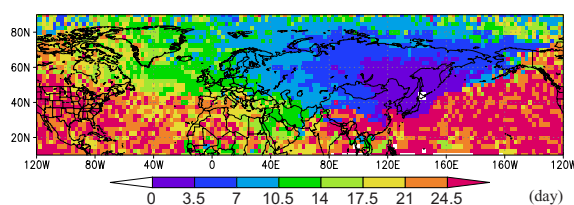
Fig. 9 Spatial distribution of the time scale of air parcel's displacement from interested areas toward the Hokkaido region in January, averaged for the period of 1980-2003.
