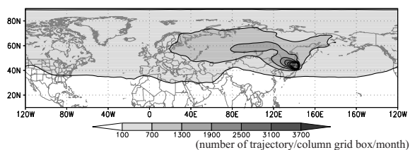
Fig. 7 Distribution of the 25day backward trajectories of air parcels that arrived over the Hokkaido region in January, averaged for the period of 1980-2003. Contours greater than 100 are indicated, with a contour interval of 600.
