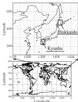
Fig. 1 Global map and location map for the Hokkaido and Kyushu regions in Japan. Air parcel's trajectories arriving at the Hokkaido (42-45N, 141-144E) and Kyushu (31-34N, 129-132E) regions were calculated.
