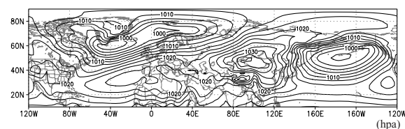
Fig. 5 The same as in Fig.4, except for the Kyushu region.
