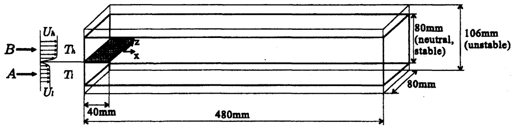
Fig. 4: The computational domain for a thermally stratified mixing layer.
