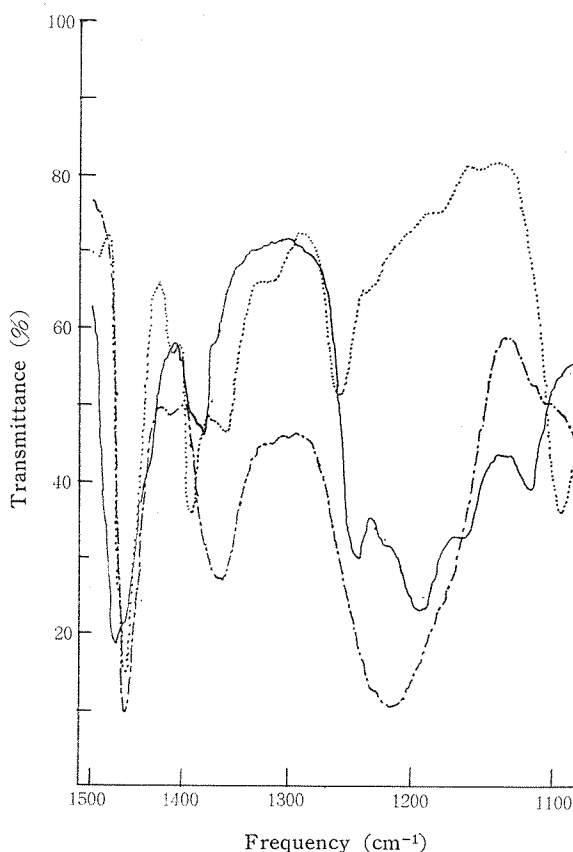
Fig. 3a. Absorption spectra of poly-AN (.....), AN-VS copolymer (-·-·-·-), and sodium VS in nujol (————).
