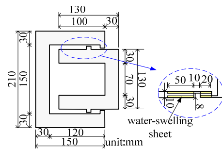
Fig. 8 The detail of the acrylic H-H joint.
