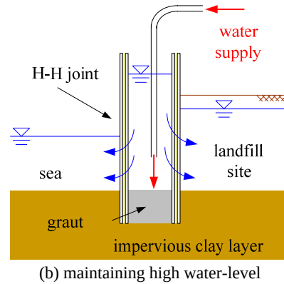
Fig. 6 Leachate control technologies using H-H joint at coastal landfill site.
