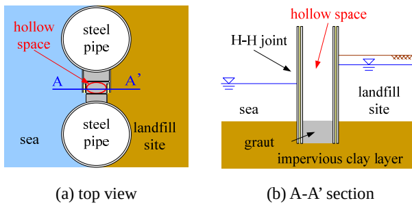
Fig. 5 Hollow space generated at H-H joint.
