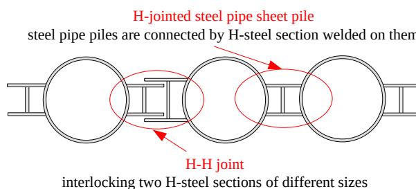
Fig. 3 H-joint SPSP with H-H joint.
