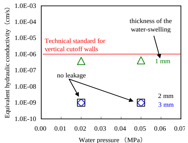
Fig. 10 Measured equivalent hydraulic conductivity for H-jointe.
