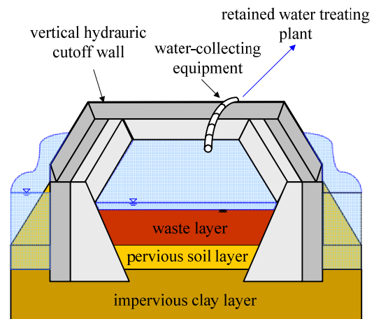
Fig. 1 Vertical hydraulic cutoff walls.
