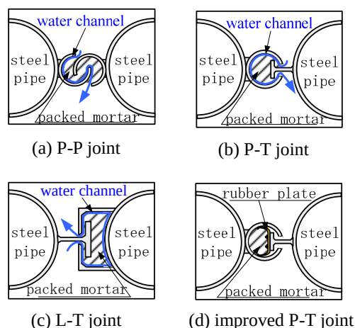
Fig. 2 Traditional joints of SPSP.
