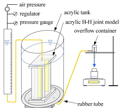
Fig. 7 A layout of testing apparatus.
