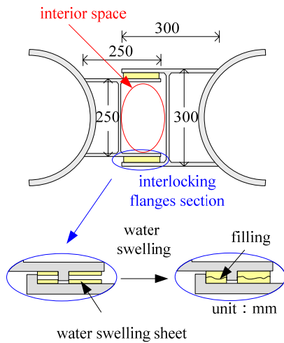
Fig. 4 Water shielding treatment in H-H joint.
