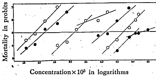
Fig. 1. Concentration-mortality curves of the larvae of Barathra brassicae L. to \gamma -BHC emulsion applied by dipping method. From left to right: 1, 2, 3, 4, 5 and the 6th instars.
