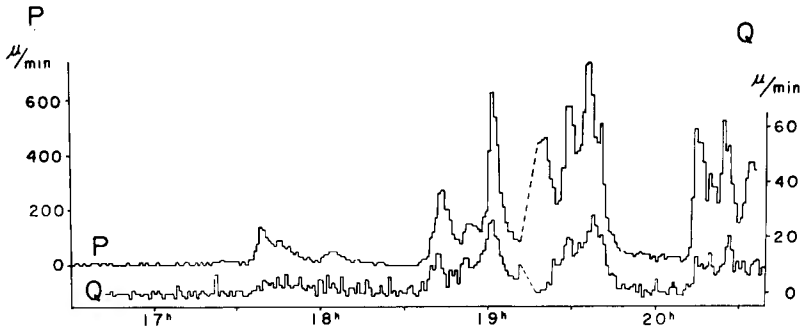
Fig. 4. Hydrograph of the runoff from the entire litter layer (Q) and the rainfall intensity (P) measured on June 9, 1961.
