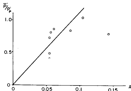
Fig. 10. Correlation between the parameter A in Table 3 and the ratio \bar{P}/P' .
