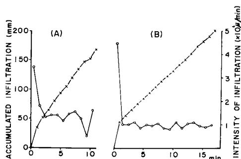
Fig. 14. The time change of the infiltration capacity measured by buffered infiltrometer on Oct. 22 (graph A) and on Oct. 23 (graph B), 1964. circle: infiltration capacity, cross: accumulated curve of infiltration capacity.
