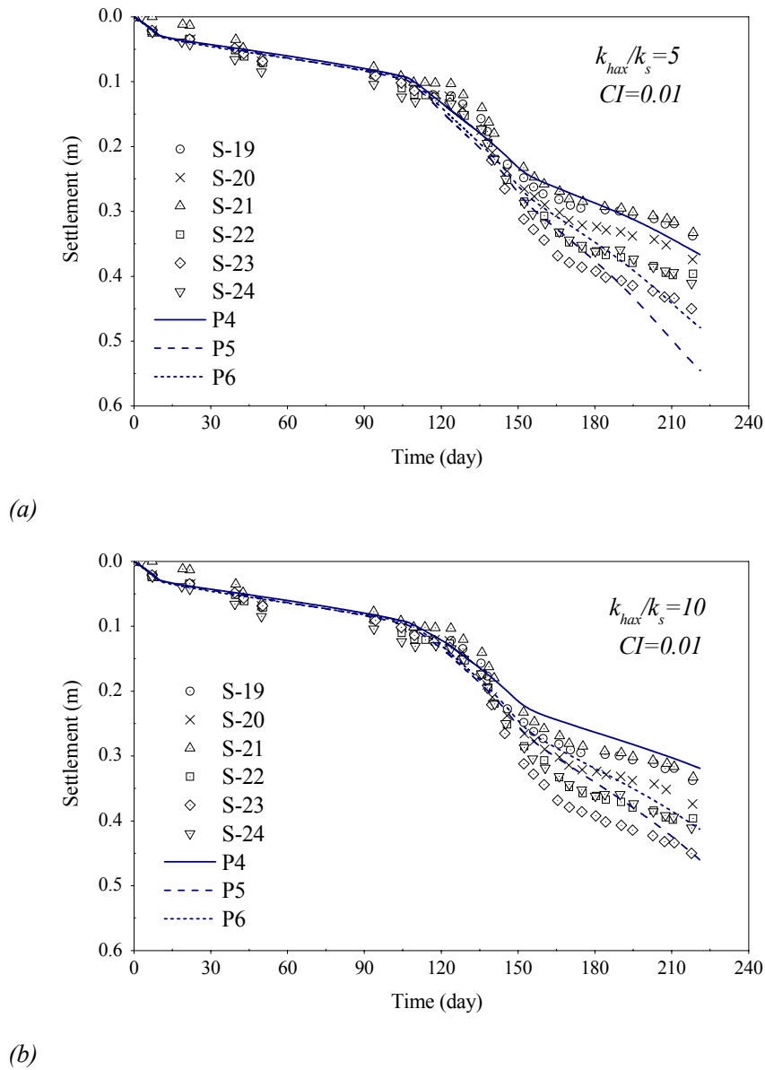
Figure 3.8. Settlement-time profiles at the ground level for the points under +7.0 m preloading; (a) k_{hax}/k_s = 5 , and (b) k_{hax}/k_s = 10 , (S19-S24 the field data points, P4-P6 the predicted data points).
