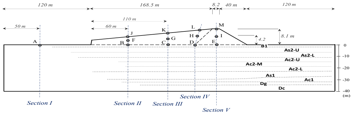
Figure 5.18. Location of the reference points for the nodal outputs within the sketch of the super levee and ground layers.
