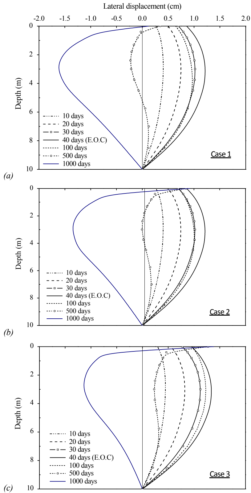
Figure 2.16. Lateral displacements under the toe of the embankment during and after construction.
