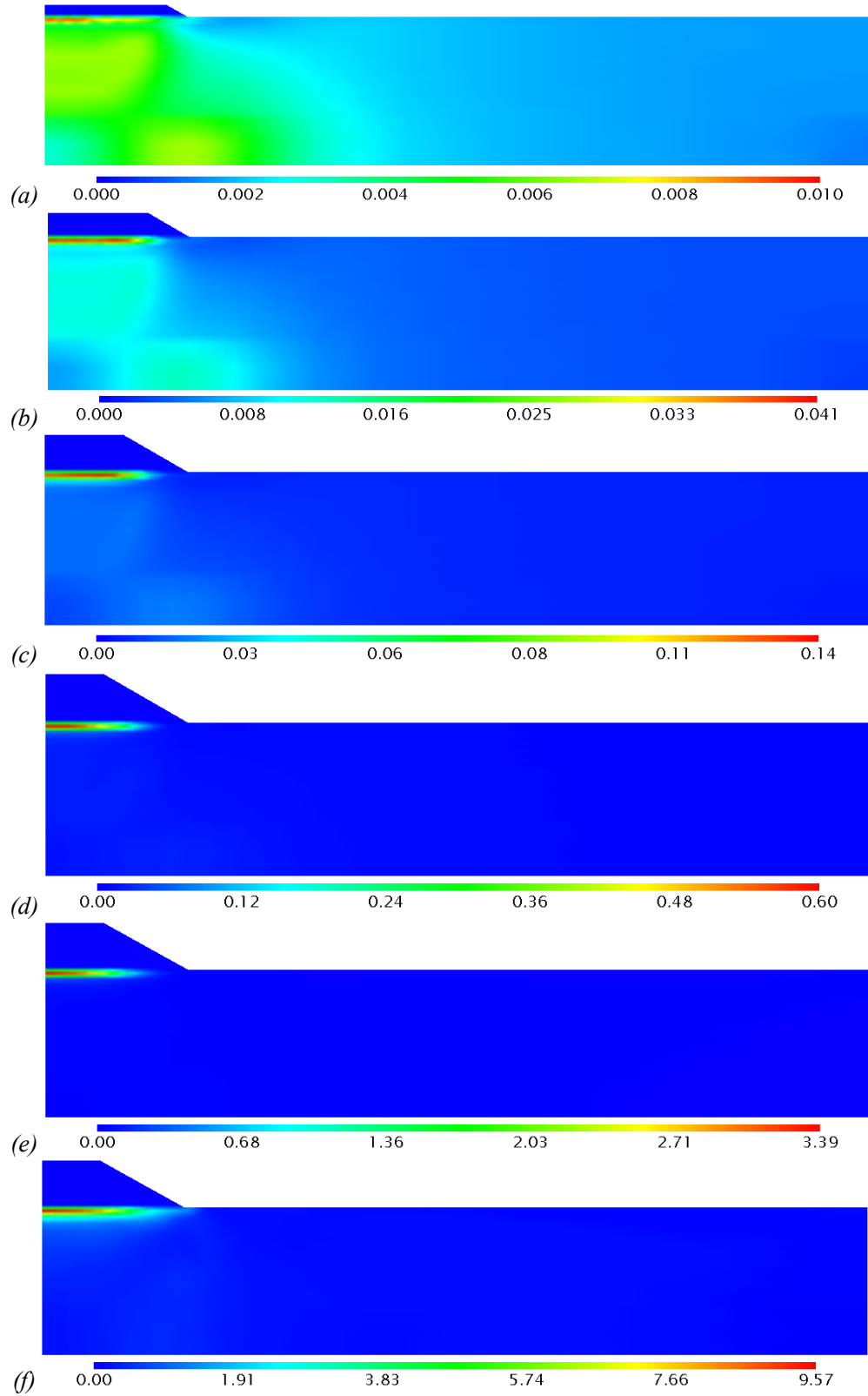
Figure 2.19. Viscoplastic shear strain contours for Case 1 on various days: (a) 10 days, (b) 20 days, (c) 30 days, (d) 40 days, (e) 100 days, and (f) 1000 days (legend unit: %).
