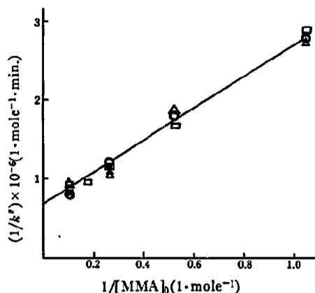
Fig. 7 The dependence of the slopes of zero-order plots (Fig. 4) on initial concentrations of MMA
