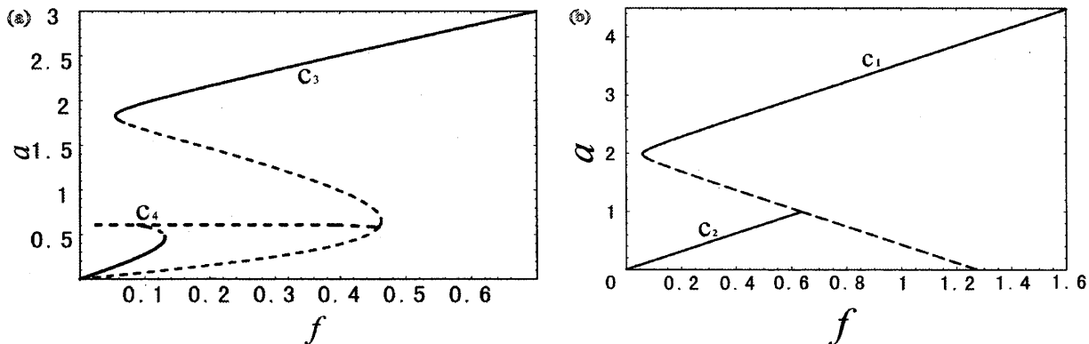
Figure 1: Response curves for \delta = 0.05 , \omega = 0.6 and \omega_0 = 1 near (0,0) and (\pm\sqrt{1-\alpha^2}, 0) in (3) and (4), respectively, the solid lines represents the stable and the dashed line marks the unstable periodic solutions: (a) response curve c_3 and c_4 for \alpha = 0.5 and (b) response curve c_1 and c_2 for \alpha = 0.0 , respectively.
