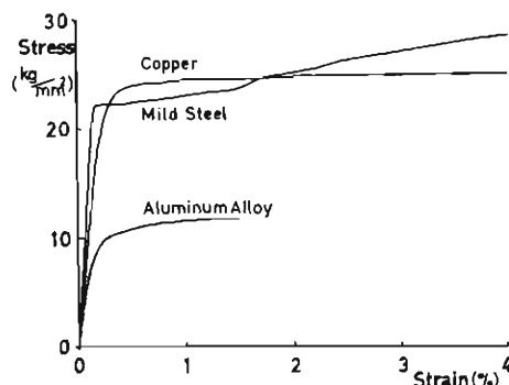
Fig. 6. Stress-strain relations.
