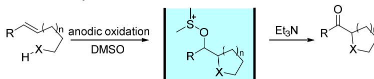
Scheme 1. Oxidation of Alkenes by Integration of Electrochemical Method and Chemical Method via Alkoxysulfonium Ions.
