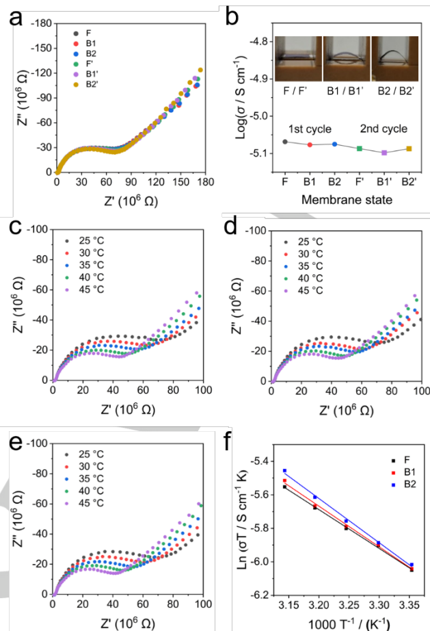
Figure 4. (a) Nyquist plots of \text{Cu}_2(\text{NiTCPP}) membrane at 25 °C and 98% RH in various bending states; F: flat, B1: 1st bending state ( R = 5.3 mm), B2: 2nd bending state ( R = 3.8 mm); F', B1', and B2' are equivalent to those of F, B1, and B2, respectively, in the second cycle. (b) Proton conductivity ( \sigma ) of \text{Cu}_2(\text{NiTCPP}) membrane at 25 °C and 98% RH in various bending states (the inset shows the photographs of each bending state). Temperature dependence of the Nyquist plots of \text{Cu}_2(\text{NiTCPP}) membrane in the (c) F, (d) B1, and (e) B2 states at 98% RH. (f) Arrhenius plots of \sigma of \text{Cu}_2(\text{NiTCPP}) membrane in various bending states.
