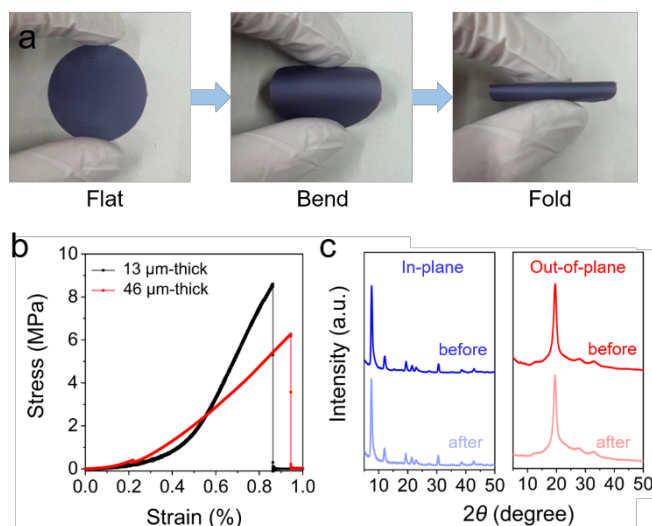
Figure 3. (a) Bending resistance test of \text{Cu}_2(\text{NiTCPP}) free-standing membrane with a thickness of 8 \mu\text{m} . (b) Tensile stress–strain curves of the membranes with the thickness of 13 \mu\text{m} (black) and 46 \mu\text{m} (red). (c) In-plane and out-of-plane XRD patterns of the membrane before (blue/red) and after (pale blue/pale red) bending, as shown in Figure 3a.
