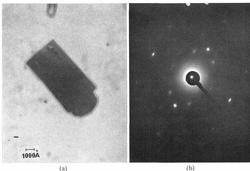
Fig. 8. (a) Electron micrograph, (b) diffraction pattern of the particle heated at 400°C.
