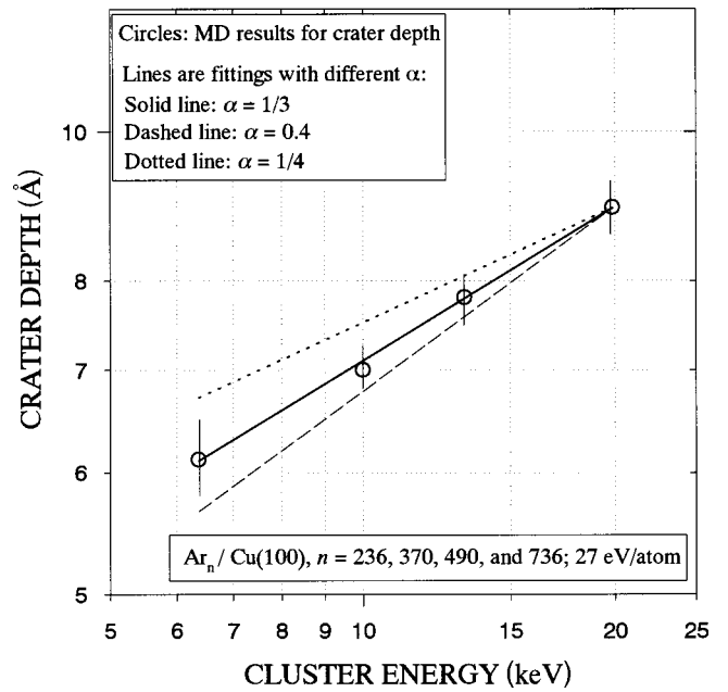
FIG. 3. Crater depth calculated by molecular dynamics for \text{Ar}_n ( n = 236, 370, 490 , and 736 ) cluster ion impact with energy of 27 eV/atom on a Cu(100) surface (circles), the straight line corresponds to the E^{1/3} power law. For comparison, the power-law dependencies with the exponents \alpha = 0.4 (dotted line) and 0.25 (dashed line) are also given.
