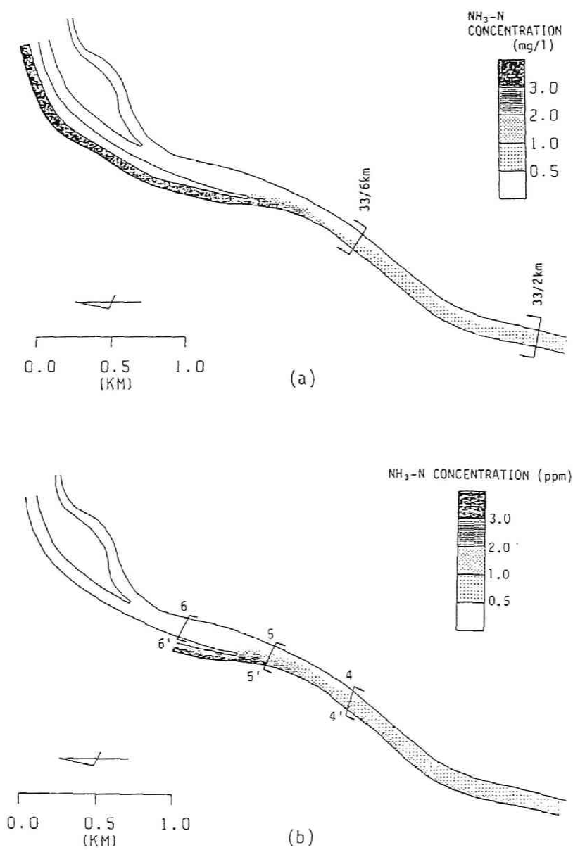
Figure 9.3.3: Spreading of NH 3 -N concentration simulated in (a) 62-0904 Test, and (b) 61-1028 Test.
