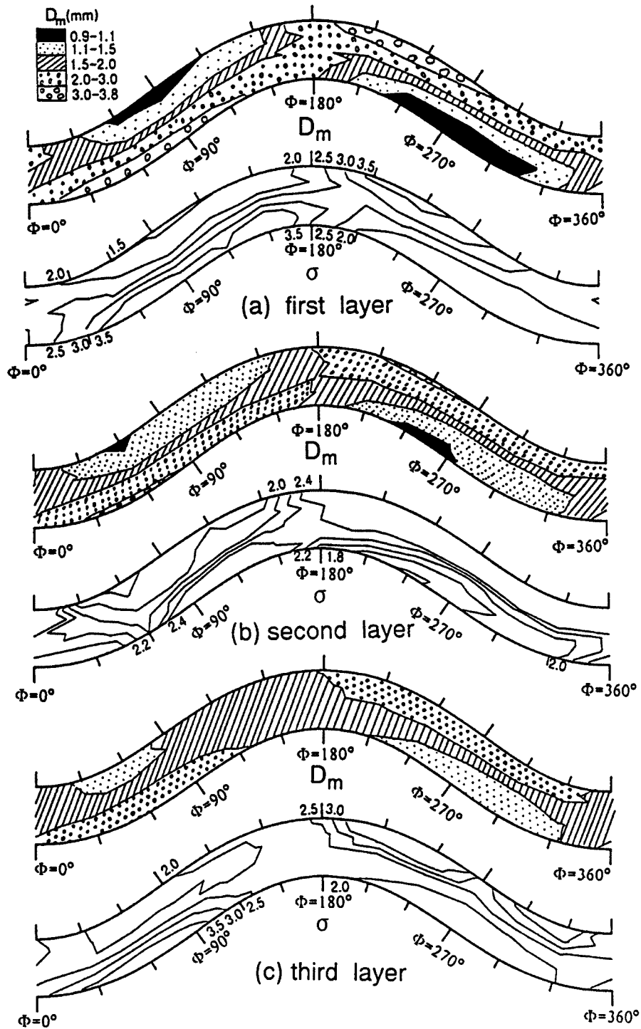
Fig. 8. Experimental results of grain size distribution of the bed material after sorting. (case 2, Q=3.6(1/s) )
