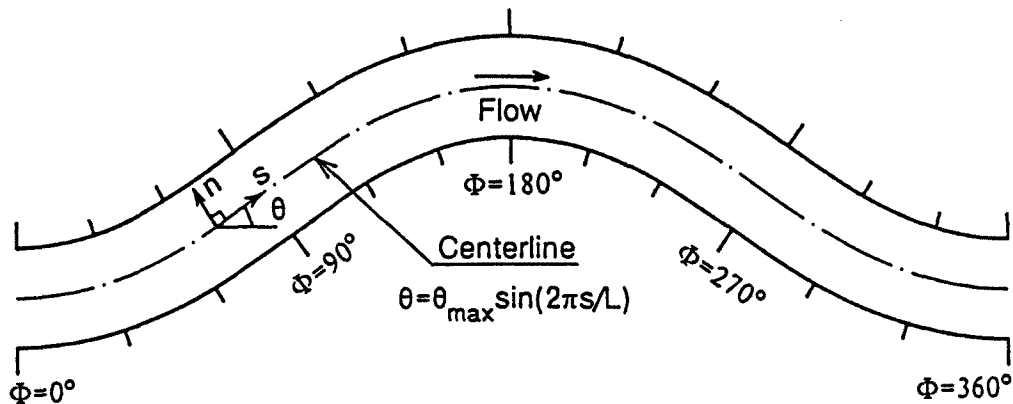
Fig. 2. Definition diagram of the experimental channel.
