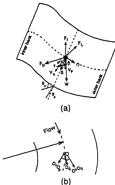
Fig. 1. (a) Forces on a sediment particle. (b) Paths taken by the sediment particles.
