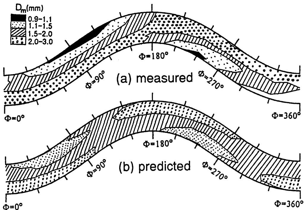
Fig. 15. Comparison of measured and predicted mean grain size distribution of surface layer in a meandering channel. (case 1: Q=1.2(l/s) , D_m=1.74(mm) , \sigma=2.2 )
