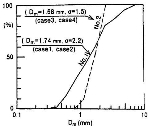
Fig. 3. Grain size distribution of sediment for the experiments.
