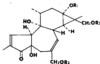
16-hydroxy-12-desoxy- phorbol esters (XVII, XVIII)
