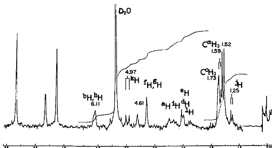
Fig. III-10. The pmr spectrum of IV(90 MHz, C_6D_6N ).
