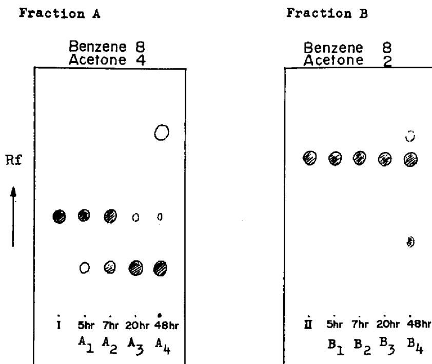
Fig. III-13. Thin layer chromatograms of products on transesterification and acetylation. Fraction A 1 ~A 4 : fractions obtained by transesterification of I. Fraction B 1 ~B 4 : fractions obtained by acetylation of Fraction A 1 ~A 4 .
