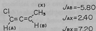
Fig. IV-7. Long-range coupling of 5.
