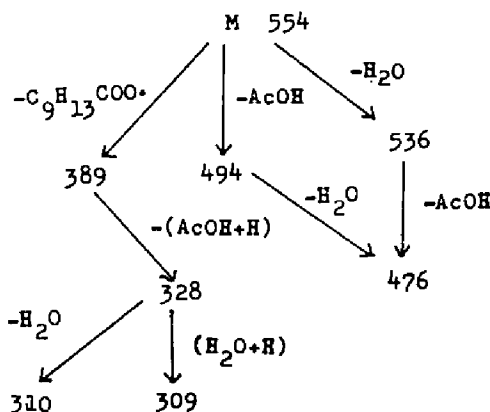
Fig. III-12. The schema of significant fragmentations of I in the mass spectrometry.
