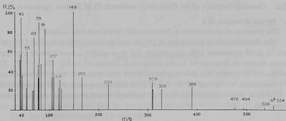
Fig. III-3. The mass spectrum of I.
