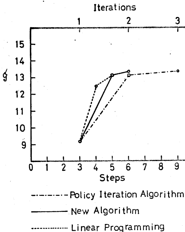
Fig. 7. 3. Comparison among the three algorithms for the taxicab problem.
