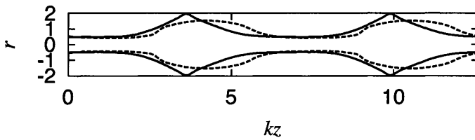
図 5: Breakup profiles for different Wb when H = 2 (solid lines) and 3 (broken lines), where Wb = 100 in (a) and Wb = 1000 in (b).
