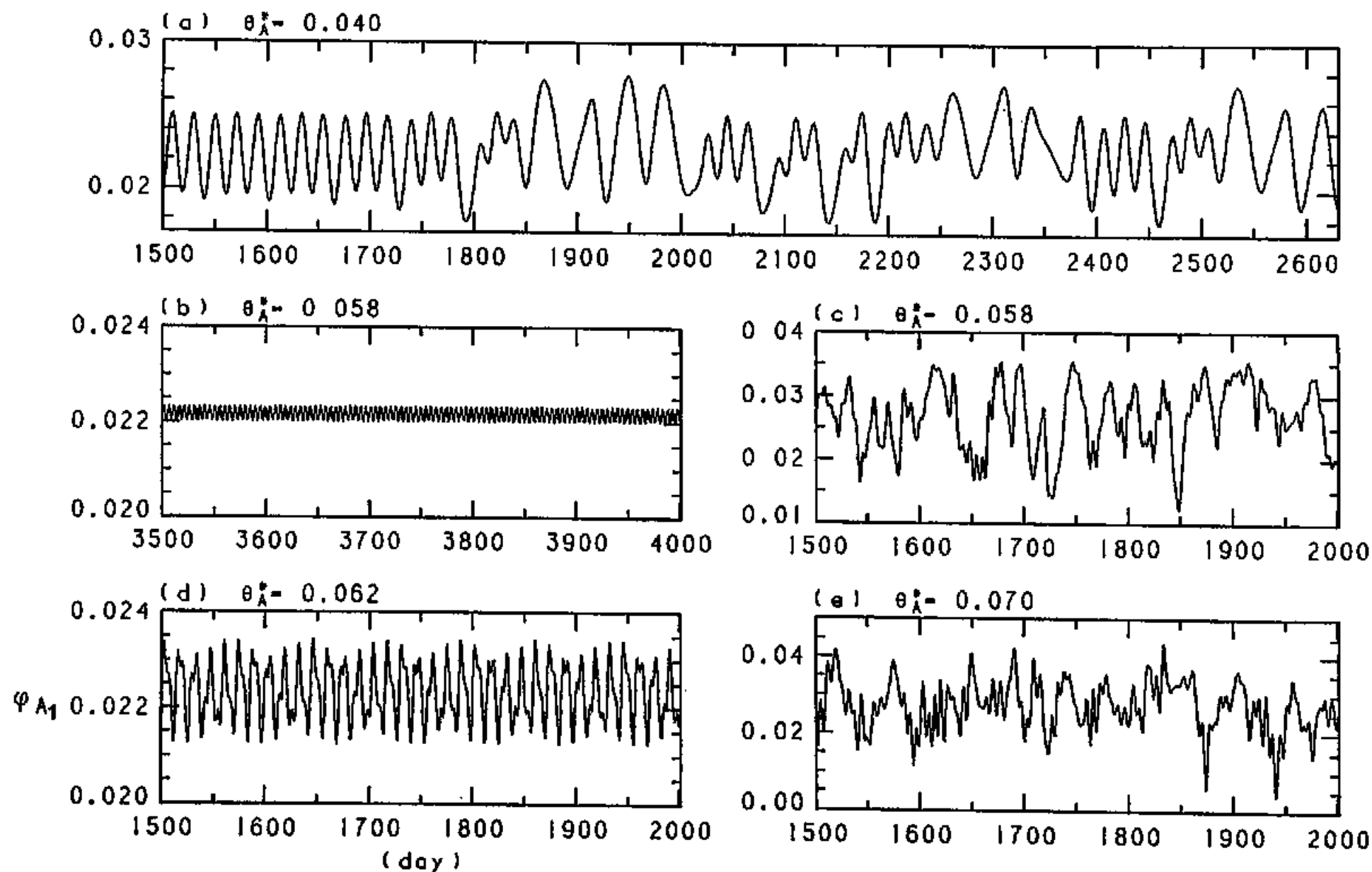
Fig.10. Time evolution of \varphi_{A1} component in some numerical solutions. The abscissa denotes the day from the beginning of the record with asymptotic behavior.
