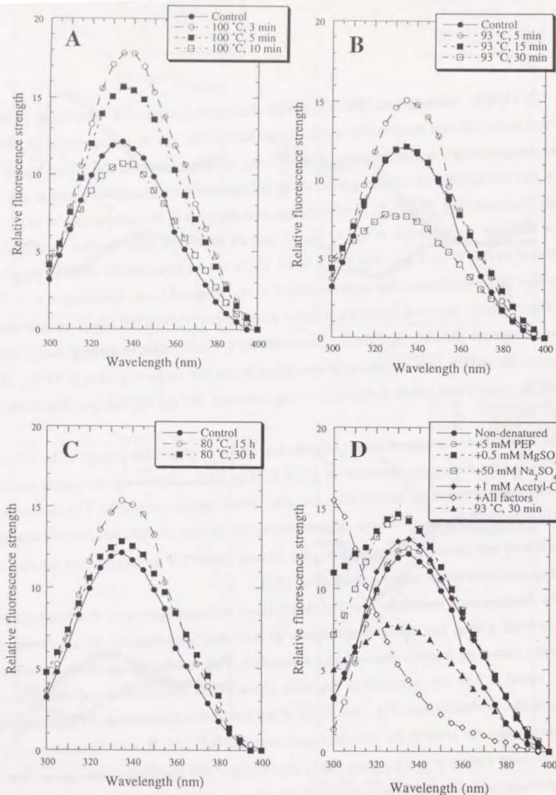
Fig. 16. The Trp fluorescence emission spectra of the enzyme denatured at 100 °C (A), 93 °C (B) and 80 °C (C). The enzyme (9 \mu gPEPC/ml) in the Tris-HCl (pH 8.0) containing 10% (wt/vol) glycerol was incubated for several periods of time at each temperature, and cooled on ice. Then the spectrum of the sample was measured at room temperature with the spectrofluorophotometer. In an attempt to examine the effect of the extrinsic thermostabilization factors, the spectra were measured under the denaturation at 93 °C for 30 min in the presence or absence of the factors (D). No apparent change was found in the spectra with each factor but the spectrum with all factors was unsettled at every experiment. All the spectra were contracted with the spectra of the incubation solution without the enzyme.
