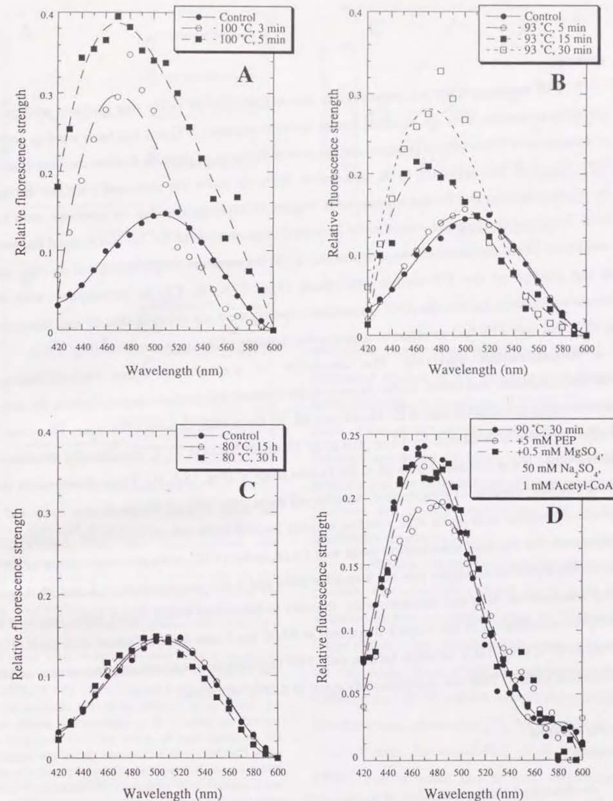
Fig. 17. The ANS fluorescence emission spectra of the enzyme denatured at 100 °C (A), 93 °C (B) and 80 °C (C). The enzyme (9 \mu gPEPC/ml) in the Tris-HCl (pH 8.0) containing 10% (wt/vol) glycerol was incubated for several periods of time at each temperature, and cooled on ice. Then ANS was added to the incubation solution at a final concentration of 0.1 \mu M. After 4 h of incubation at 4 °C, the spectrum of the solution with ANS was measured at room temperature with the spectrofluorophotometer. In an attempt to examine the effect of the extrinsic thermostabilization factors, the spectra were measured under the denaturation at 93 °C for 30 min in the presence or absence of the factors (D). No apparent change was found in the spectra with the factors between before and after the thermodenaturation. All the spectra were contracted with the spectra of the incubation solution without the enzyme.
