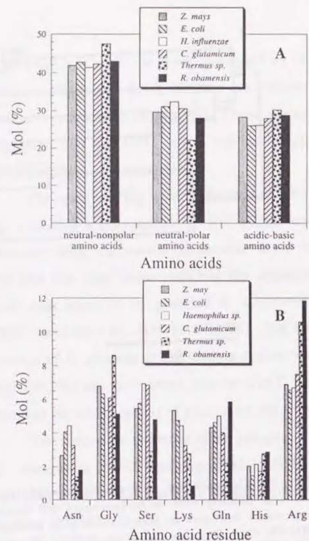
Fig. 24. The amino acid compositions of representative bacterial and eucaryal PEPCs. (A) The comparison of three distinct physicochemical groups of amino acids. The neutral-nonpolar amino acids contain Ala, Ile, Leu, Met, Phe, Pro and Val, the neutral-polar amino acids contain Asn, Cys, Gln, Gly, Ser, Thr, Trp and Tyr, and the acidic or basic amino acids include Arg, Asp, Glu, His and Lys. (B) The comparison of some amino acid compositions that demonstrate relatively high or low contents in R. obamensis PEPC. The amino acid compositions in this figure were found to be different between R. obamensis PEPC and all other mesophilic PEPCs. Hence, some amino acid compositions were similar between R. obamensis PEPC and Thermus PEPC.
