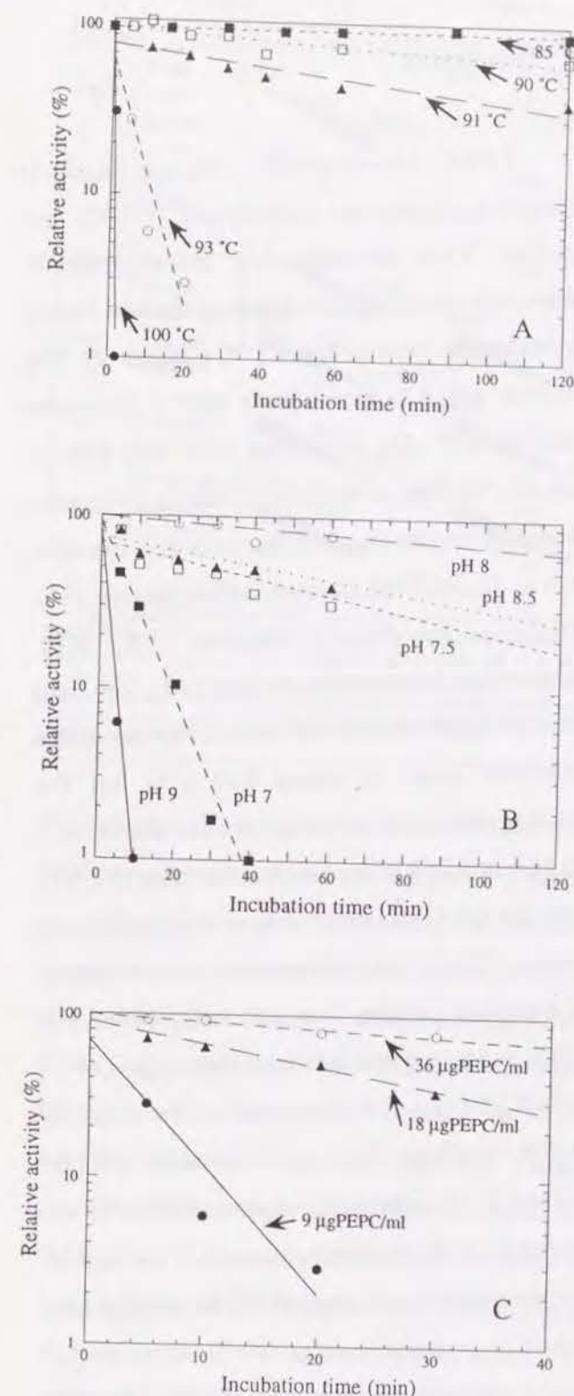
Fig. 10. The effects of temperature, pH and enzyme concentration on thermostability. (A) The thermoinactivation of R. obamensis PEPC at various temperatures. The enzyme was incubated at various temperatures at a concentration of 9 µg PEPC/ml in the incubation buffer (50 mM Tris-HCl containing 10% glycerol, pH 8.0) for different periods of time. The thermoinactivation was terminated by cooling the aliquots on ice and the residual activity was measured at 75 °C at pH 8.0. The activity before the thermoinactivation was set to 100%. (B) The effect of pH on the thermostability of R. obamensis PEPC. The enzyme was incubated at 91 °C and a concentration of 9 µg PEPC/ml. The pH of the incubation buffer indicated in this figure was the value adjusted at 25 °C and the value was found to decrease to the extent of 1.3 at 91 °C. The activity at each pH value before the thermoinactivation was set to 100%. (C) The effect of enzyme concentration on the thermostability of R. obamensis PEPC. The enzyme was incubated at 93 °C and pH 8.0 at 9, 18 or 36 µg PEPC/ml. In this experiment, the total protein concentration was standardized to a concentration of 72 µg/ml in all cases by the compensation of bovine serum albumin (BSA). The activity at each enzyme concentration before the thermoinactivation was set to 100%.
