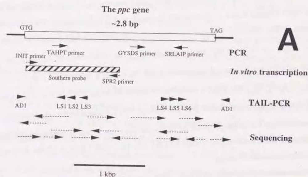
Fig. 19. The sequence strategy (A) and nucleotide and deduced amino acid sequences of the ppc gene of R. obamensis (B). (A) The partial fragment of the ppc gene was amplified by polymerase chain reaction (PCR) using the primers with the sequences 5'-TSACTGCYCAACSGA-3' (TAHP primer) and 5'-GTCCAGGCSATSACCCASGGGATGG-3' (SRLAIP primer), and directly sequenced on both strand by the dideoxynucleotide chain termination method using DNA sequencer Model 373As (Applied Biosystem Inc.). Based on the sequence of the fragment, the thermal asymmetric interlaced (TAIL) PCR was carried out to determine the sequence of the unknown regions adjacent to the known sequence of the gene [110]. The primers for the TAIL PCR are described in Materials and Methods and indicated in (B). The amplified fragments containing 5'- and 3'-flanking regions of the ppc gene were directly sequenced on both strand by the dideoxynucleotide chain termination method. The shadow box indicates a 1.3 kb of RNA probe complementary to the fragment amplified with the INIT and SPR2 primers shown in (B). (B) Nucleotide and amino acid sequences are numbered starting with the putative initiation codon and N-terminal amino acid residue. The primers used for the PCR, TAIL PCR, southern analysis and cloning are indicated with arrows above the nucleotide sequence, corresponding to the sequence of the primers. The putative Shine-Dalgarno sequence is double underlined. The underlined amino acid sequences are the partial sequences of peptides produced from the purified R. obamensis PEPC by V8 endopeptidase of Staphylococcus aureus and determined by Edman degradation method (Takai et al. unpublished data). The asterisk indicates the stop codon.
