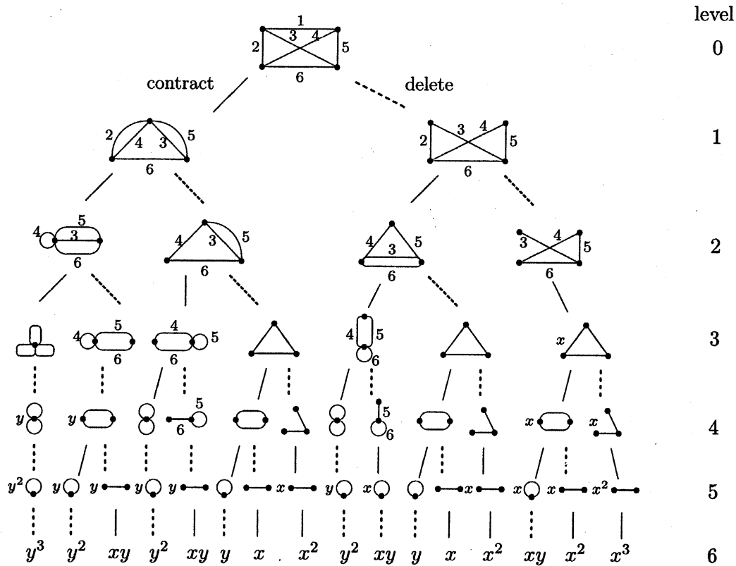
Figure 1: Expansion tree for complete graph K_4
