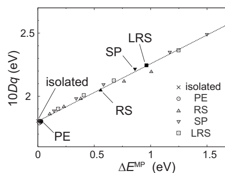
FIG. 5. Relationship between the difference between the Madelung potential acting on e_g and t_{2g} orbitals and the magnitude of 10Dq at the ground state. The Co-O bond length in the \text{CoO}_6^{9-} cluster is fixed at 1.92 Å. The reduction/enhancement factor of the Madelung potential, Q , is set at 0, 0.25, 0.5, 0.75, 1, 1.25, and 1.5. Filled marks denote the values with Q=1 .
