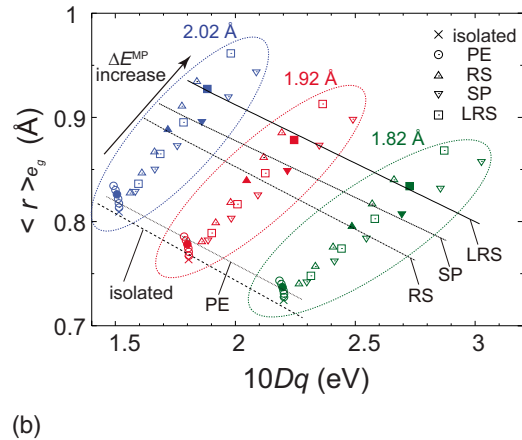
FIG. 10. (Color online) (a) Difference in partial charge distributions of the e_g orbitals between PE and LRS with R=1.92 Å, \Delta\rho = \rho_{\text{LRS}} - \rho_{\text{PE}} . (b) Averaged radial distance of e_g orbitals, \langle r \rangle_{e_g} , calculated for different Madelung potential and R , as a function of 10Dq . Q is set at 0, 0.25, 0.5, 0.75, 1, 1.25, and 1.5. Filled marks denote the values with Q=1 and the dotted curves enclose the results with the same R .
