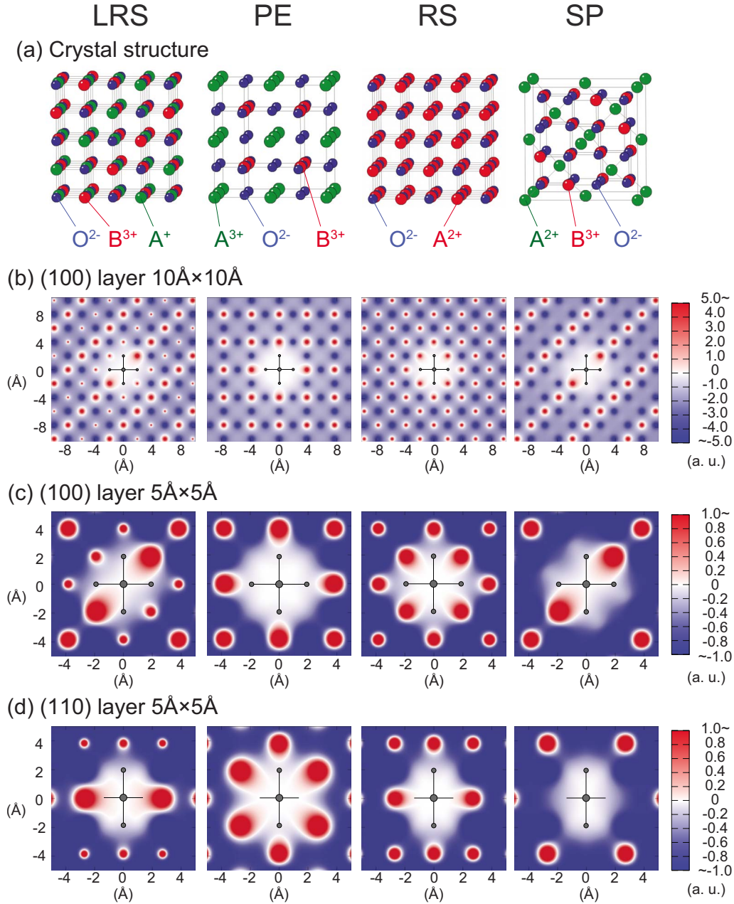
FIG. 3. (Color online) (a) Crystal structures of layered rock salt (LRS), perovskite (PE), rock salt (RS), and spinel (SP). [(b), (c)] Madelung potential around the CoO_6^{9-} cluster for each structure on the (100) plane. (d) The same potential on the (110) plane.
