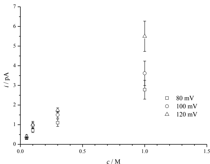
Fig. 3 Concentration dependence of the single channel current. Applied membrane potential: 80 mV, 100 mV and 120 mV.
