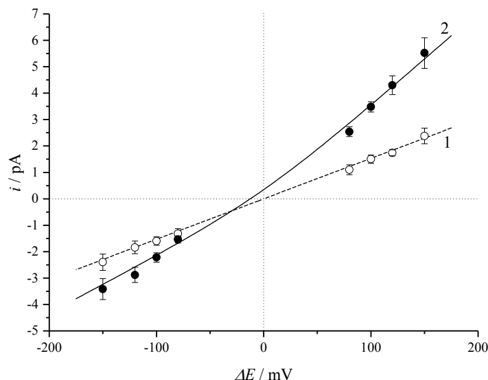
Fig. 2 Dependence of the single channel current on the membrane potential. The concentration of KCl in W1 and W2: 0.3 M (○). The concentration of KCl in W1 and W2: 1.0 M (W1) and 0.3 M (W2) (●). T = 298 \pm 1 K. Curves 1 and 2: calculated curves fitted to the experimental results.
