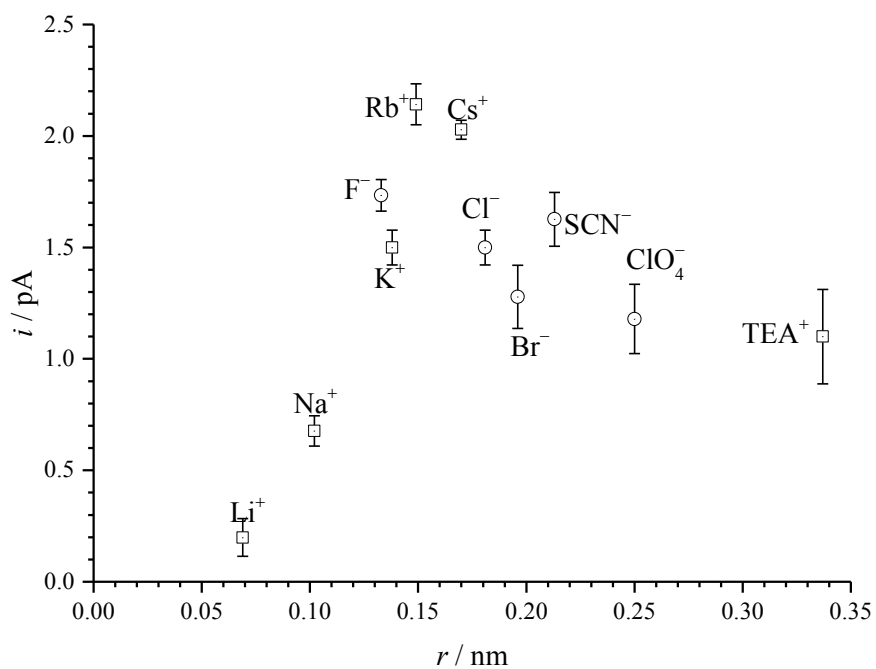
Fig. 2 The dependence of single-channel currents at +120mV on the ionic radii of ions.
