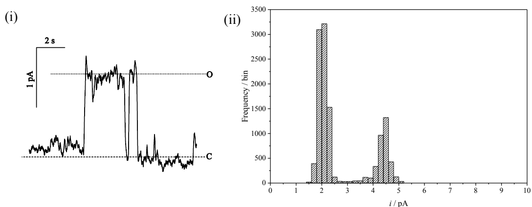
Fig. 1 (i) Single channel recording of KAT1 channel in 0.3 M KCl. The applied potential was +0.1 V. C indicates the closed state and O the open state. (ii) Amplitude histogram constructed from the data for measurement at +0.1 V.
