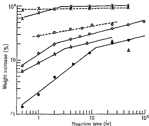
Fig. 5 Reaction rates of esterification with trans -crotonic (○), methacrylic (●), acrylic (△) and \beta -methylcrotonic (x) acid, at 30°C wood; — untreated ..... EDA-treated
