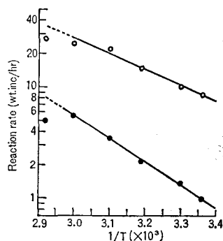
Fig. 6 Temperature dependence of reaction rates for trans -crotonylation (○) and methacrylation (●)
