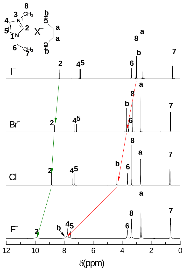
Figure 2. ^1H NMR spectra of [C_2C_{1im}]X \cdot EG ( X = F, Cl, Br and I ) complexes at 20 °C. The arrows show the trend of the related chemical shift as function of anion size.
