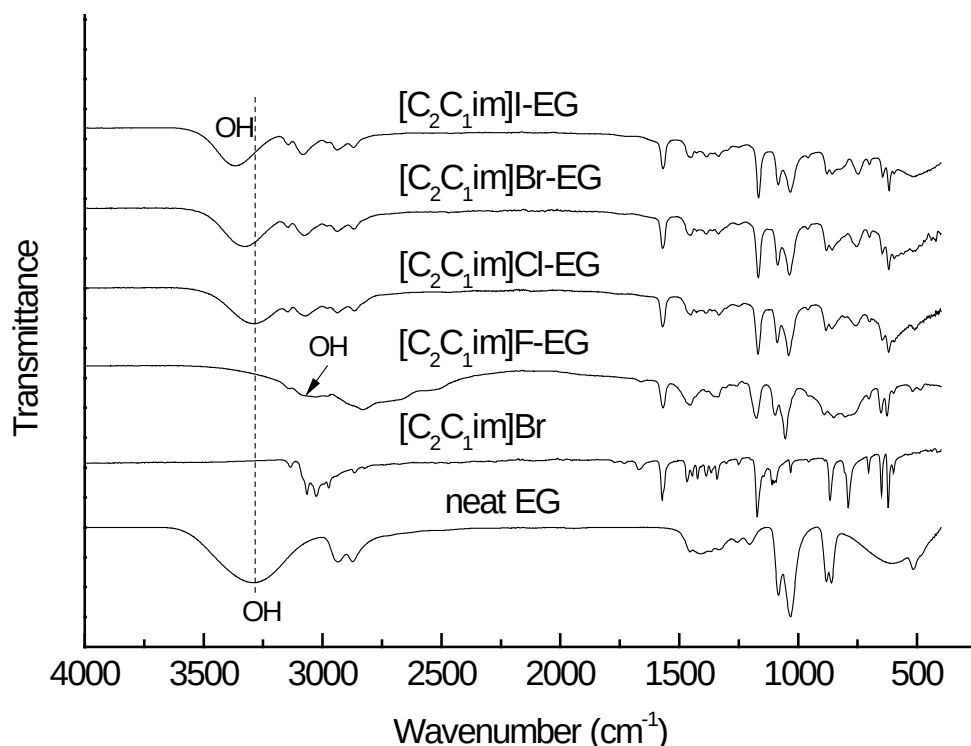
Figure 4. Infrared spectra of [\text{C}_2\text{C}_{1\text{im}}]\text{X}\cdot\text{EG} ( \text{X} = \text{F}, \text{Cl}, \text{Br} and \text{I} ), [\text{C}_2\text{C}_{1\text{im}}]\text{Br} , and pure EG at 20 °C .
