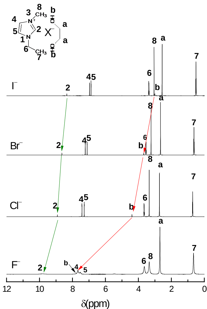
Figure 5. ^1\text{H} NMR spectra of [\text{C}_2\text{C}_1\text{im}]\text{X} \cdot \text{EG} ( \text{X} = \text{F}, \text{Cl}, \text{Br} , and \text{I} ) after 24-hour deuteration with \text{D}_2\text{O} at 20\text{ }^\circ\text{C} . The arrows show the trend of the chemical shift for Hb and H2 along with the change of anion.
