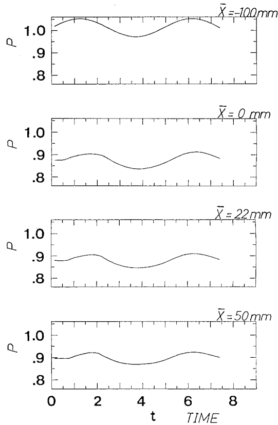
Fig. 18 Propagation of pressure waves for \bar{p}_0 = 1.013 \times 10^5 Pa, \bar{p}_D = 0.747 \times 10^5 Pa, \bar{m}_g = 3 Nl/min and \bar{f} = 400 Hz.
