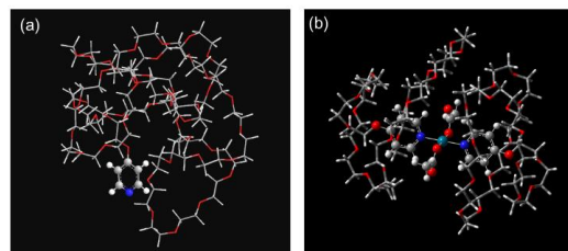
Figure 1. Optimized structures of PEG-functionalized pyridines. (a) 1c (n = 45). The pyridine ring moiety is shown as a ball and stick model. (b) \text{Pd}(\text{OAc})_2(\mathbf{1b})_2 (n = 17). The \text{Pd}(\text{OAc})_2(\text{py})_2 core is shown as a ball and stick model.
