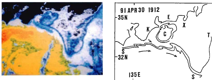
Fig. 2 Thermal pattern on the sea surface at 19h12m on 30th April 1991.
